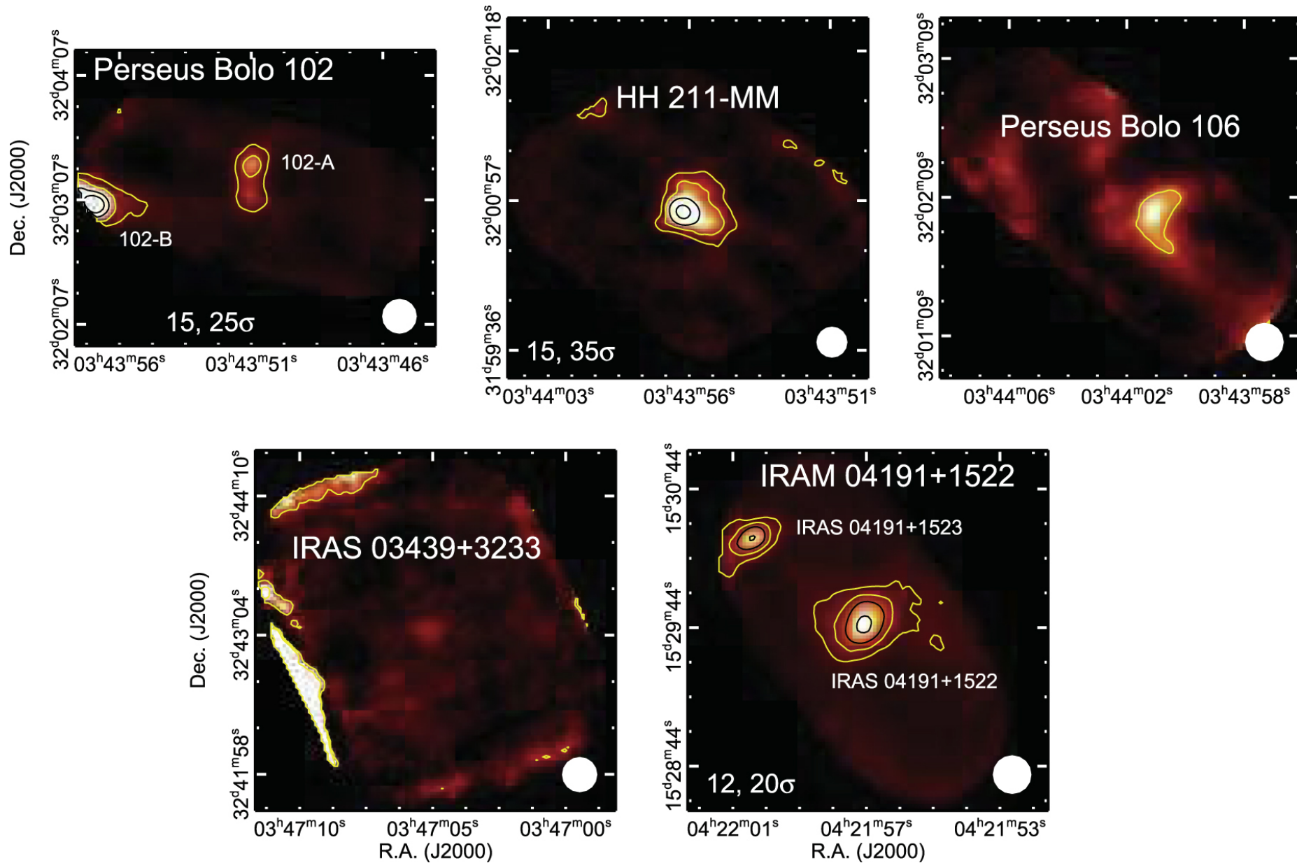
Figure 33. from A CATALOG OF LOW-MASS STAR-FORMING CORES OBSERVED WITH SHARC-II AT 350 m null 2016 AJ 152 36 doi:10.3847/0004-6256/152/2/36 https://dx.doi.org/10.3847/0004-6256/152/2/36 © 2016. The American Astronomical Society. All rights reserved.
