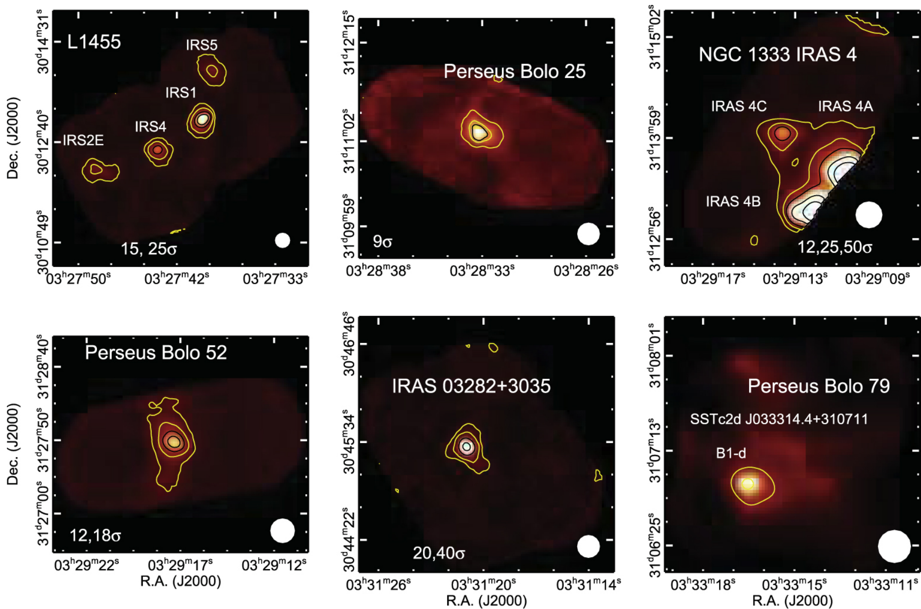
Figure 32. from A CATALOG OF LOW-MASS STAR-FORMING CORES OBSERVED WITH SHARC-II AT 350 m null 2016 AJ 152 36 doi:10.3847/0004-6256/152/2/36 https://dx.doi.org/10.3847/0004-6256/152/2/36 © 2016. The American Astronomical Society. All rights reserved.
