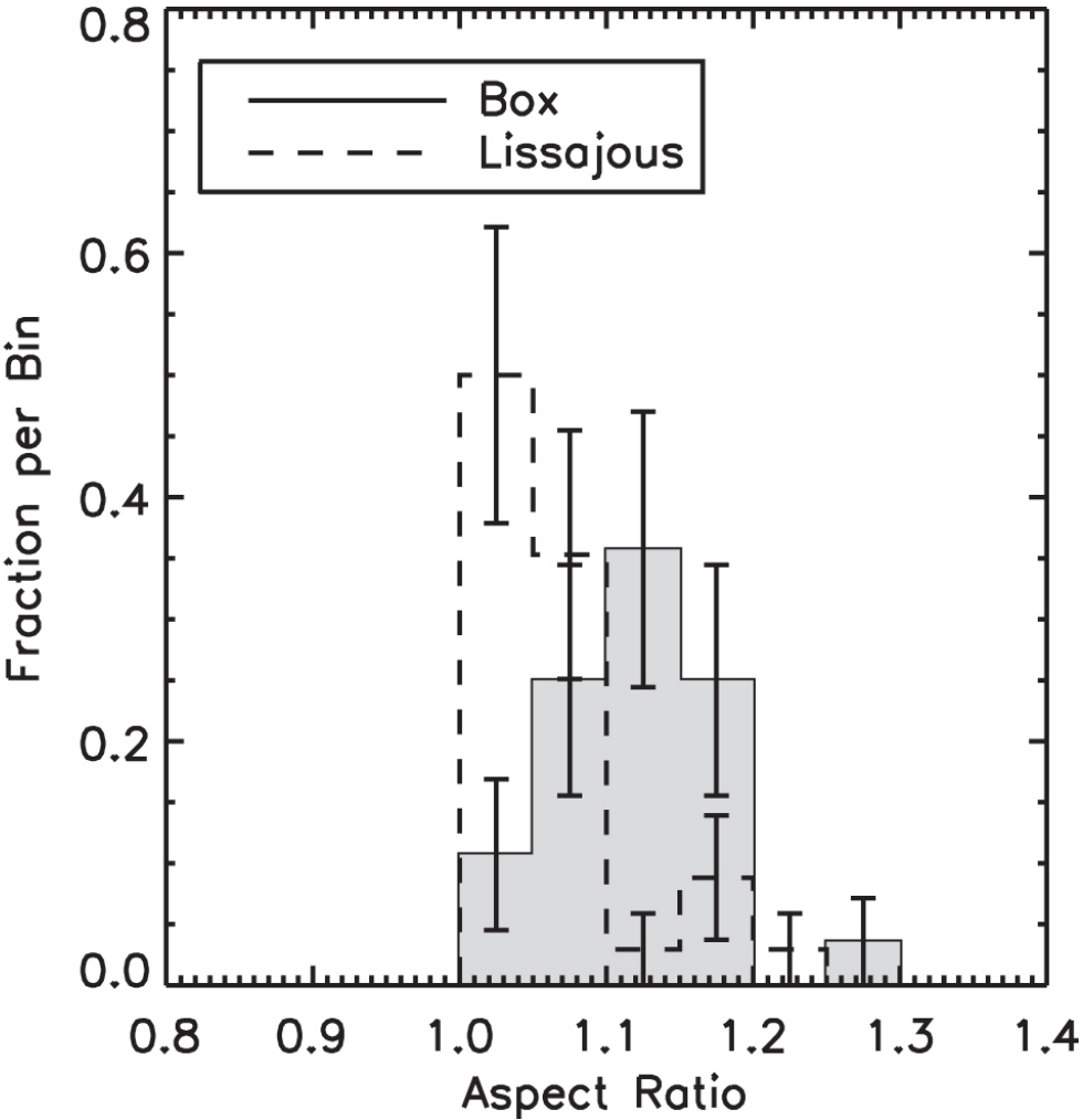
Figure 31. from A CATALOG OF LOW-MASS STAR-FORMING CORES OBSERVED WITH SHARC-II AT 350 m null 2016 AJ 152 36 doi:10.3847/0004-6256/152/2/36 https://dx.doi.org/10.3847/0004-6256/152/2/36 © 2016. The American Astronomical Society. All rights reserved.
