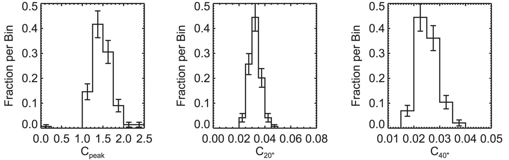
Figure 3. from A CATALOG OF LOW-MASS STAR-FORMING CORES OBSERVED WITH SHARC-II AT 350 m null 2016 AJ 152 36 doi:10.3847/0004-6256/152/2/36 https://dx.doi.org/10.3847/0004-6256/152/2/36
