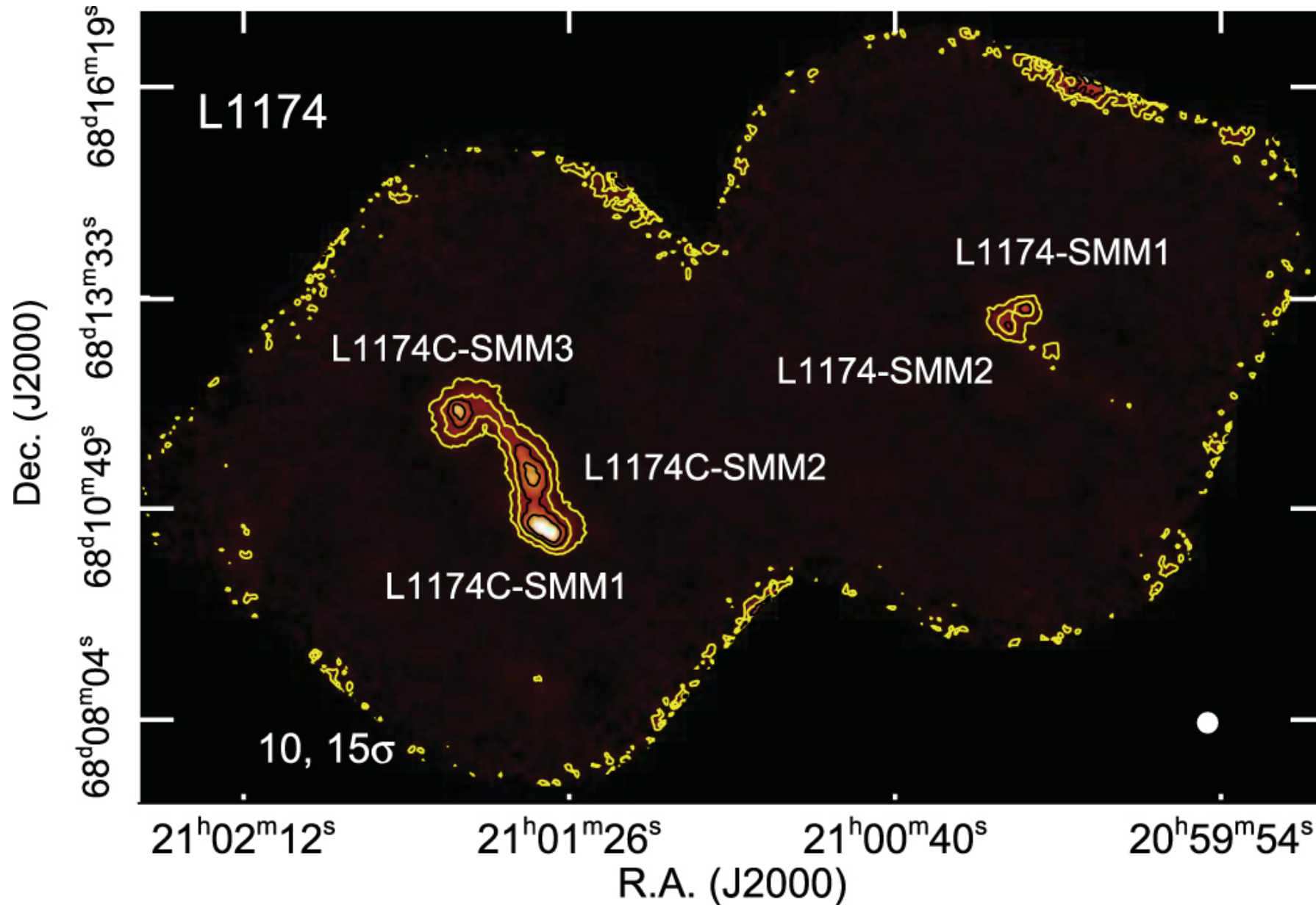
Figure 29. from A CATALOG OF LOW-MASS STAR-FORMING CORES OBSERVED WITH SHARC-II AT 350 m null 2016 AJ 152 36 doi:10.3847/0004-6256/152/2/36 https://dx.doi.org/10.3847/0004-6256/152/2/36 © 2016. The American Astronomical Society. All rights reserved.
