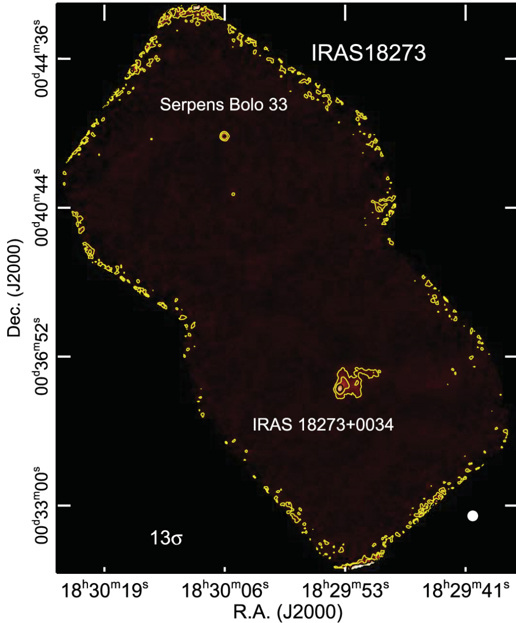
Figure 24. from A CATALOG OF LOW-MASS STAR-FORMING CORES OBSERVED WITH SHARC-II AT 350 m null 2016 AJ 152 36 doi:10.3847/0004-6256/152/2/36 https://dx.doi.org/10.3847/0004-6256/152/2/36 © 2016. The American Astronomical Society. All rights reserved.
