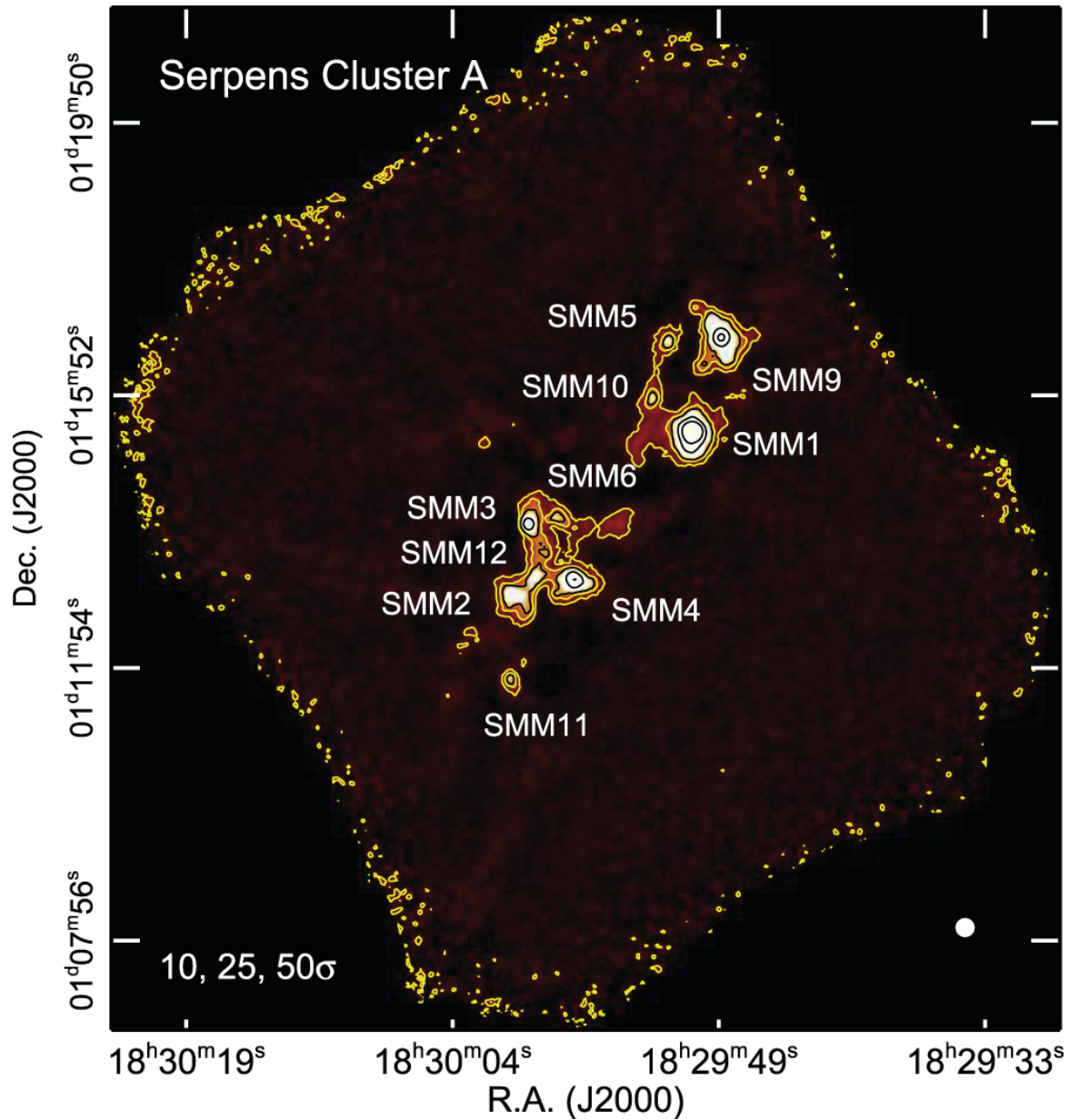
Figure 23. from A CATALOG OF LOW-MASS STAR-FORMING CORES OBSERVED WITH SHARC-II AT 350 m null 2016 AJ 152 36 doi:10.3847/0004-6256/152/2/36 https://dx.doi.org/10.3847/0004-6256/152/2/36 © 2016. The American Astronomical Society. All rights reserved.
