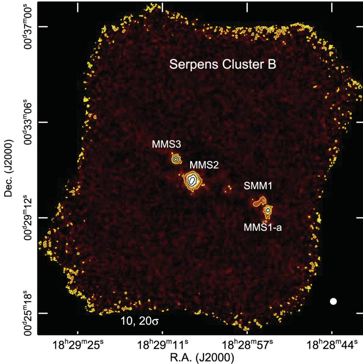
Figure 22. from A CATALOG OF LOW-MASS STAR-FORMING CORES OBSERVED WITH SHARC-II AT 350 m null 2016 AJ 152 36 doi:10.3847/0004-6256/152/2/36 https://dx.doi.org/10.3847/0004-6256/152/2/36 © 2016. The American Astronomical Society. All rights reserved.
