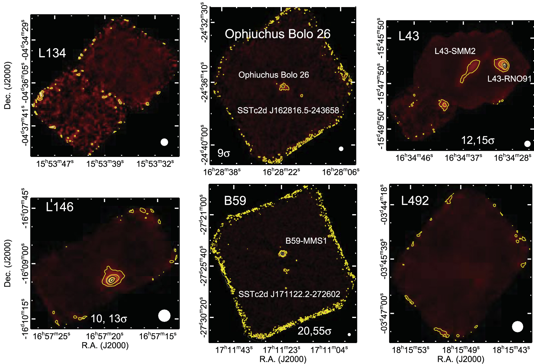
Figure 20. from A CATALOG OF LOW-MASS STAR-FORMING CORES OBSERVED WITH SHARC-II AT 350 m null 2016 AJ 152 36 doi:10.3847/0004-6256/152/2/36 https://dx.doi.org/10.3847/0004-6256/152/2/36 © 2016. The American Astronomical Society. All rights reserved.
