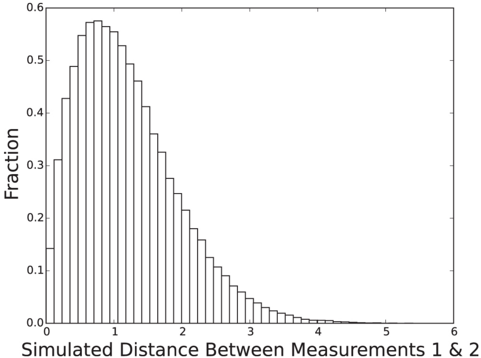
Figure 2. from A CATALOG OF LOW-MASS STAR-FORMING CORES OBSERVED WITH SHARC-II AT 350 m null 2016 AJ 152 36 doi:10.3847/0004-6256/152/2/36 https://dx.doi.org/10.3847/0004-6256/152/2/36 © 2016. The American Astronomical Society. All rights reserved.
