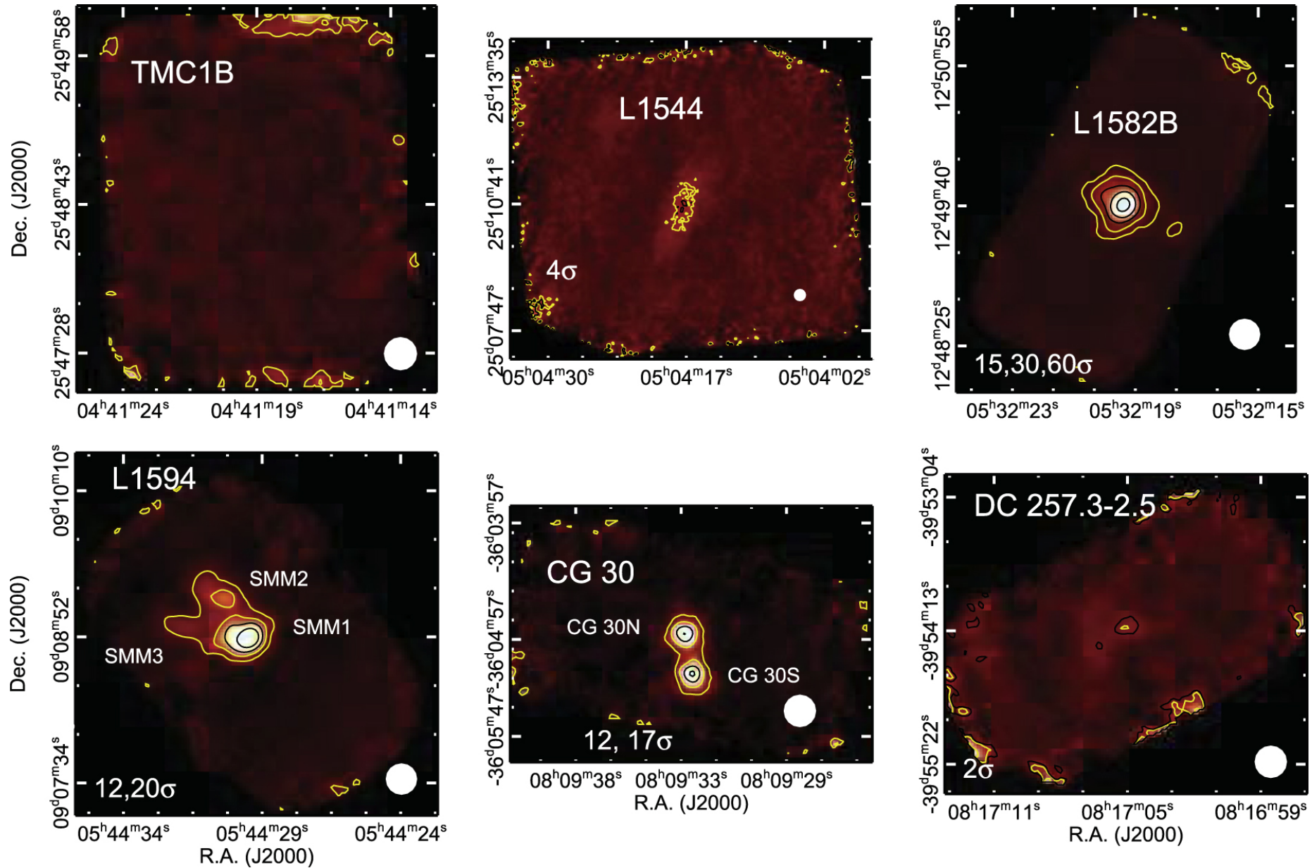
Figure 19. from A CATALOG OF LOW-MASS STAR-FORMING CORES OBSERVED WITH SHARC-II AT 350 m null 2016 AJ 152 36 doi:10.3847/0004-6256/152/2/36 https://dx.doi.org/10.3847/0004-6256/152/2/36 © 2016. The American Astronomical Society. All rights reserved.
