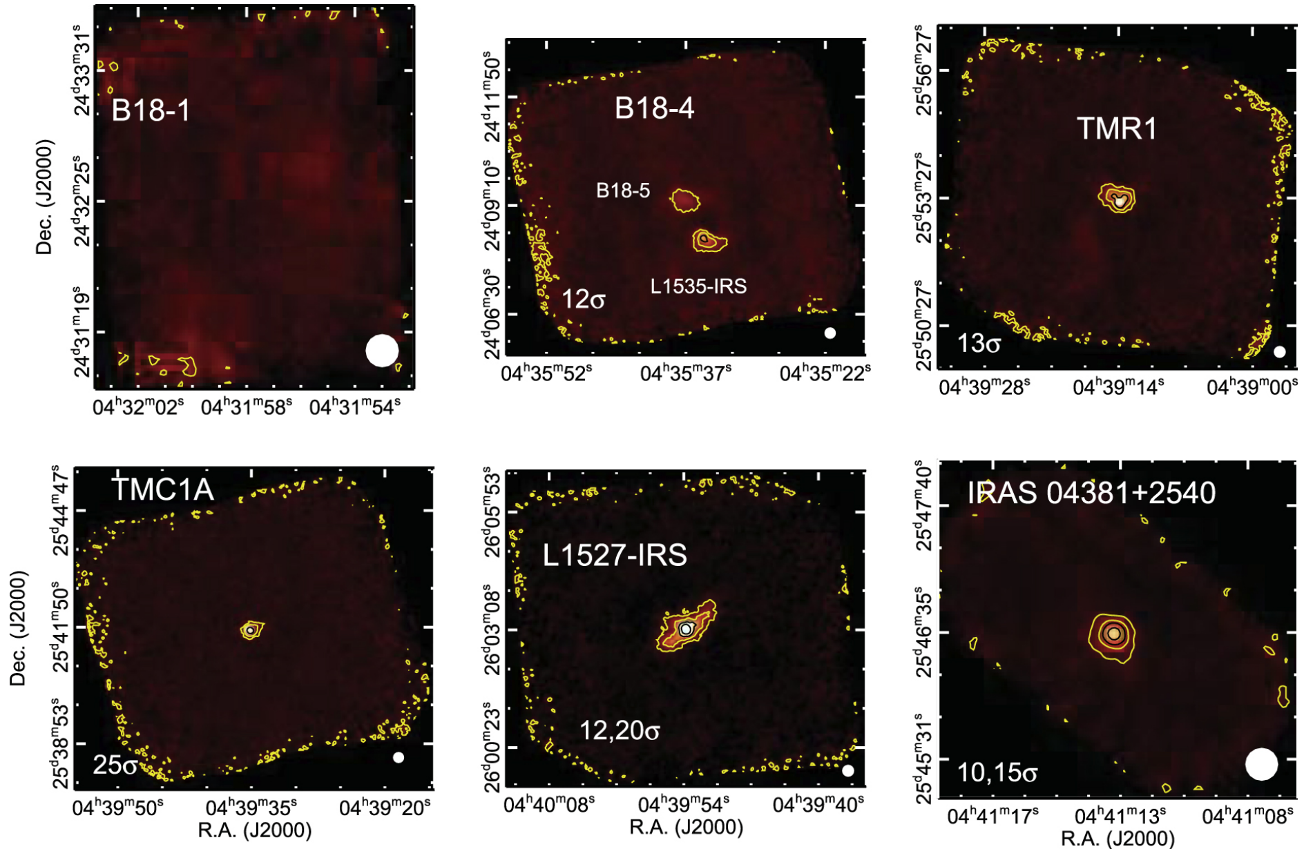
Figure 18. from A CATALOG OF LOW-MASS STAR-FORMING CORES OBSERVED WITH SHARC-II AT 350 m null 2016 AJ 152 36 doi:10.3847/0004-6256/152/2/36 https://dx.doi.org/10.3847/0004-6256/152/2/36 © 2016. The American Astronomical Society. All rights reserved.
