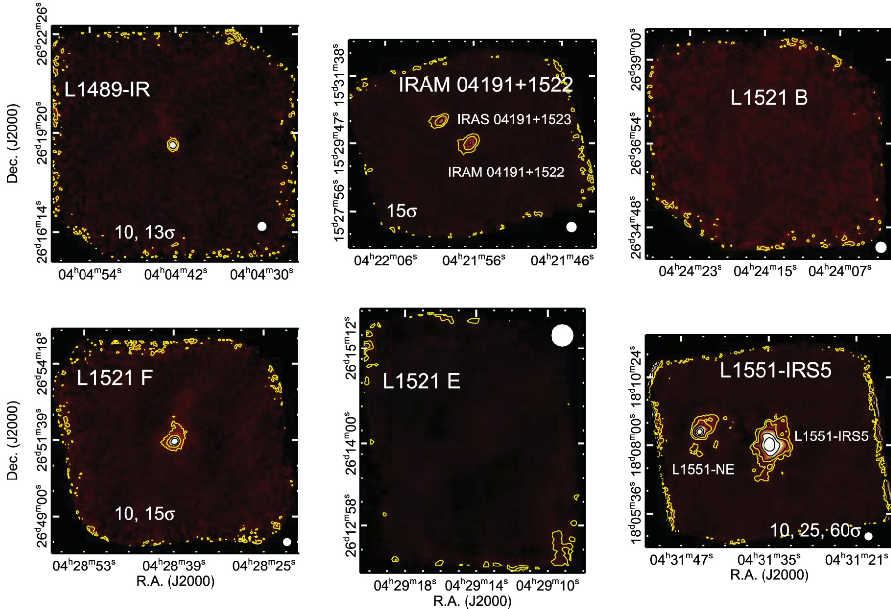
Figure 17. from A CATALOG OF LOW-MASS STAR-FORMING CORES OBSERVED WITH SHARC-II AT 350 m null 2016 AJ 152 36 doi:10.3847/0004-6256/152/2/36 https://dx.doi.org/10.3847/0004-6256/152/2/36 © 2016. The American Astronomical Society. All rights reserved.
