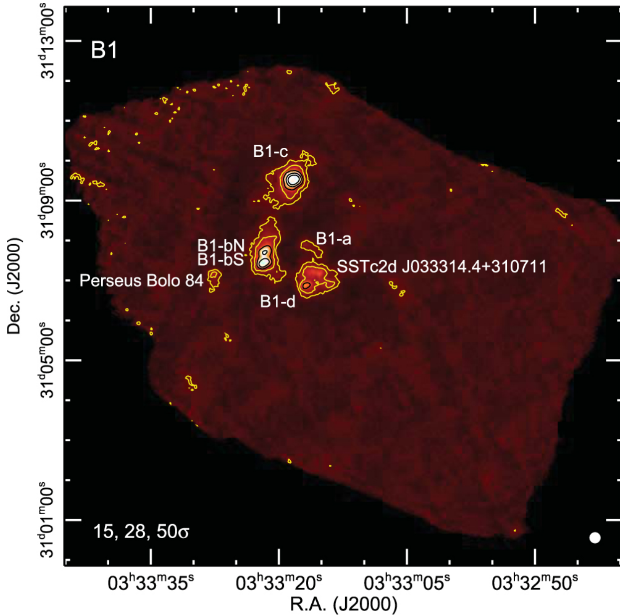
Figure 15. from A CATALOG OF LOW-MASS STAR-FORMING CORES OBSERVED WITH SHARC-II AT 350 m null 2016 AJ 152 36 doi:10.3847/0004-6256/152/2/36 https://dx.doi.org/10.3847/0004-6256/152/2/36 © 2016. The American Astronomical Society. All rights reserved.
