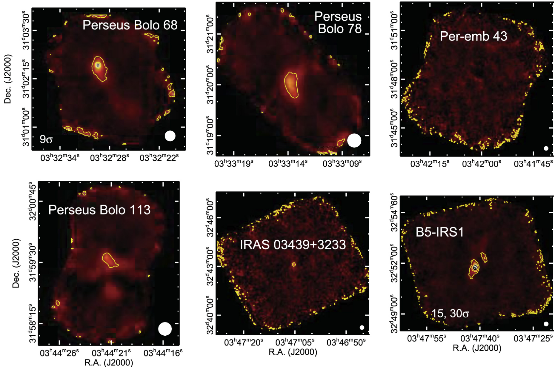
Figure 14. from A CATALOG OF LOW-MASS STAR-FORMING CORES OBSERVED WITH SHARC-II AT 350 m null 2016 AJ 152 36 doi:10.3847/0004-6256/152/2/36 https://dx.doi.org/10.3847/0004-6256/152/2/36 © 2016. The American Astronomical Society. All rights reserved.
