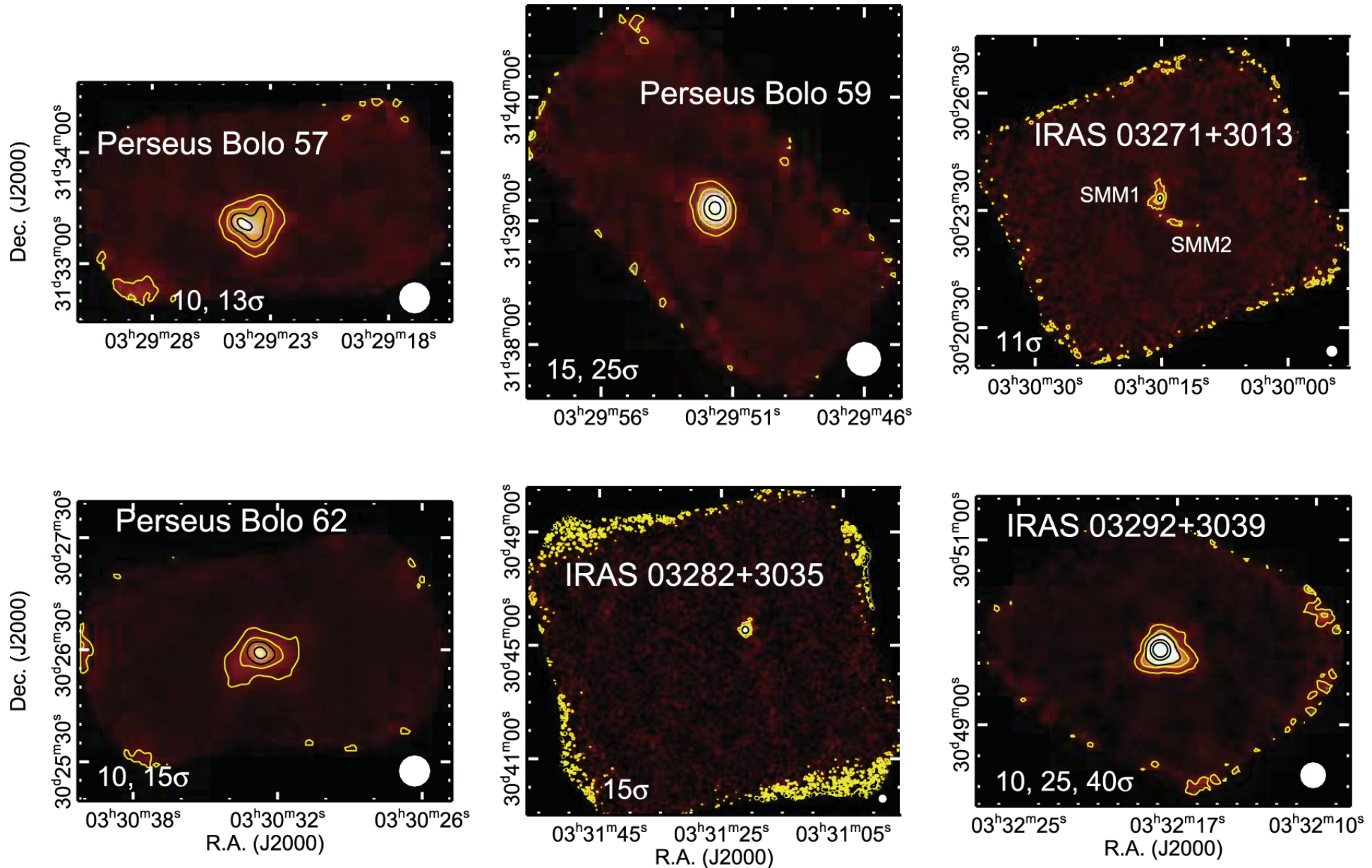
Figure 13. from A CATALOG OF LOW-MASS STAR-FORMING CORES OBSERVED WITH SHARC-II AT 350 m null 2016 AJ 152 36 doi:10.3847/0004-6256/152/2/36 https://dx.doi.org/10.3847/0004-6256/152/2/36 © 2016. The American Astronomical Society. All rights reserved.
