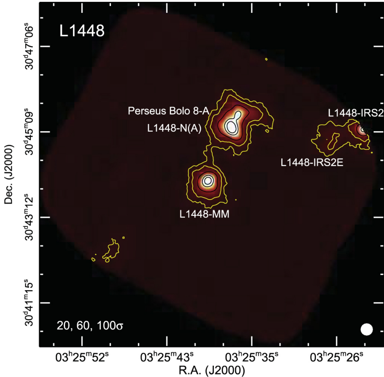
Figure 10. from A CATALOG OF LOW-MASS STAR-FORMING CORES OBSERVED WITH SHARC-II AT 350 m null 2016 AJ 152 36 doi:10.3847/0004-6256/152/2/36 https://dx.doi.org/10.3847/0004-6256/152/2/36 © 2016. The American Astronomical Society. All rights reserved.
