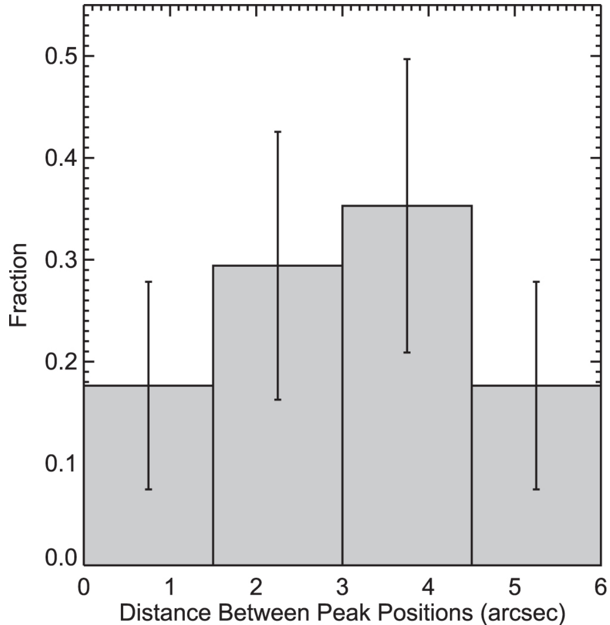
Figure 1. from A CATALOG OF LOW-MASS STAR-FORMING CORES OBSERVED WITH SHARC-II AT 350 m null 2016 AJ 152 36 doi:10.3847/0004-6256/152/2/36 https://dx.doi.org/10.3847/0004-6256/152/2/36 © 2016. The American Astronomical Society. All rights reserved.
