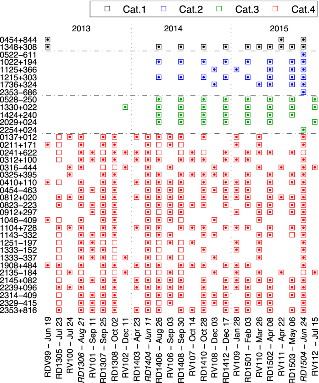
Figure 5. from IVS OBSERVATION OF ICRF2-GAIA TRANSFER SOURCES null 2016 AJ 151 79 doi:10.3847/0004-6256/151/3/79 https://dx.doi.org/10.3847/0004-6256/151/3/79 © 2016. The American Astronomical Society. All rights reserved.
