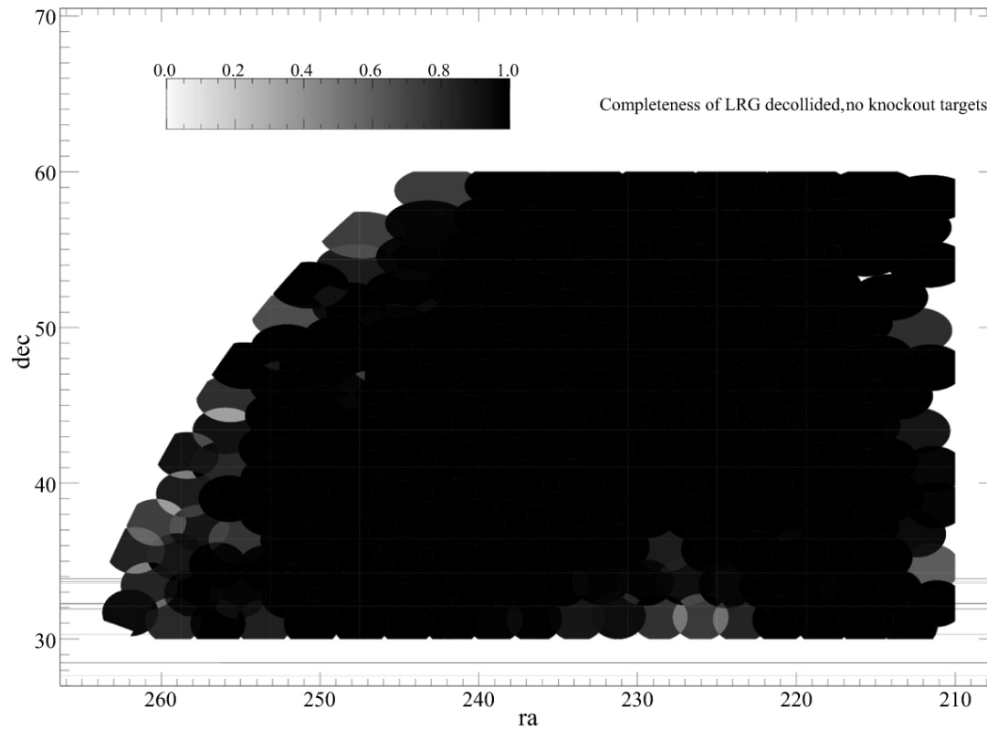
Figure 4. from THE SDSS-IV EXTENDED BARYON OSCILLATION SPECTROSCOPIC SURVEY: OVERVIEW AND EARLY DATA null 2016 AJ 151 44 doi:10.3847/0004-6256/151/2/44 https://dx.doi.org/10.3847/0004-6256/151/2/44 © 2016. The American Astronomical Society. All rights reserved.
