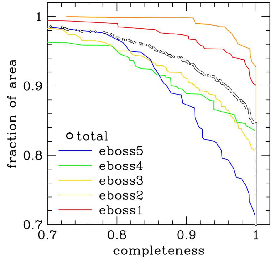
Figure 4. from THE SDSS-IV EXTENDED BARYON OSCILLATION SPECTROSCOPIC SURVEY: OVERVIEW AND EARLY DATA null 2016 AJ 151 44 doi:10.3847/0004-6256/151/2/44 https://dx.doi.org/10.3847/0004-6256/151/2/44 © 2016. The American Astronomical Society. All rights reserved.
