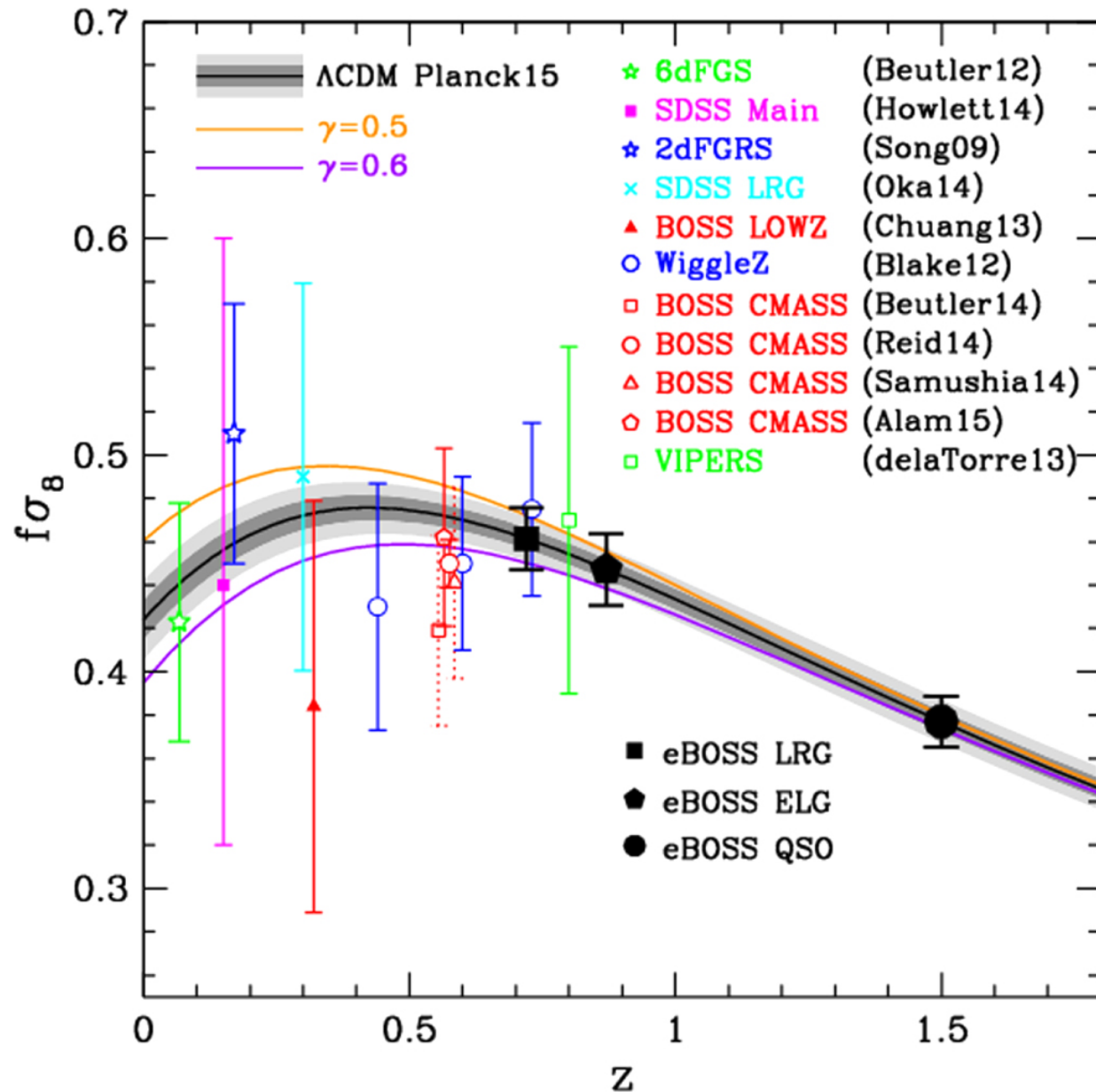
Figure 2. from THE SDSS-IV EXTENDED BARYON OSCILLATION SPECTROSCOPIC SURVEY: OVERVIEW AND EARLY DATA null 2016 AJ 151 44 doi:10.3847/0004-6256/151/2/44 https://dx.doi.org/10.3847/0004-6256/151/2/44 © 2016. The American Astronomical Society. All rights reserved.
