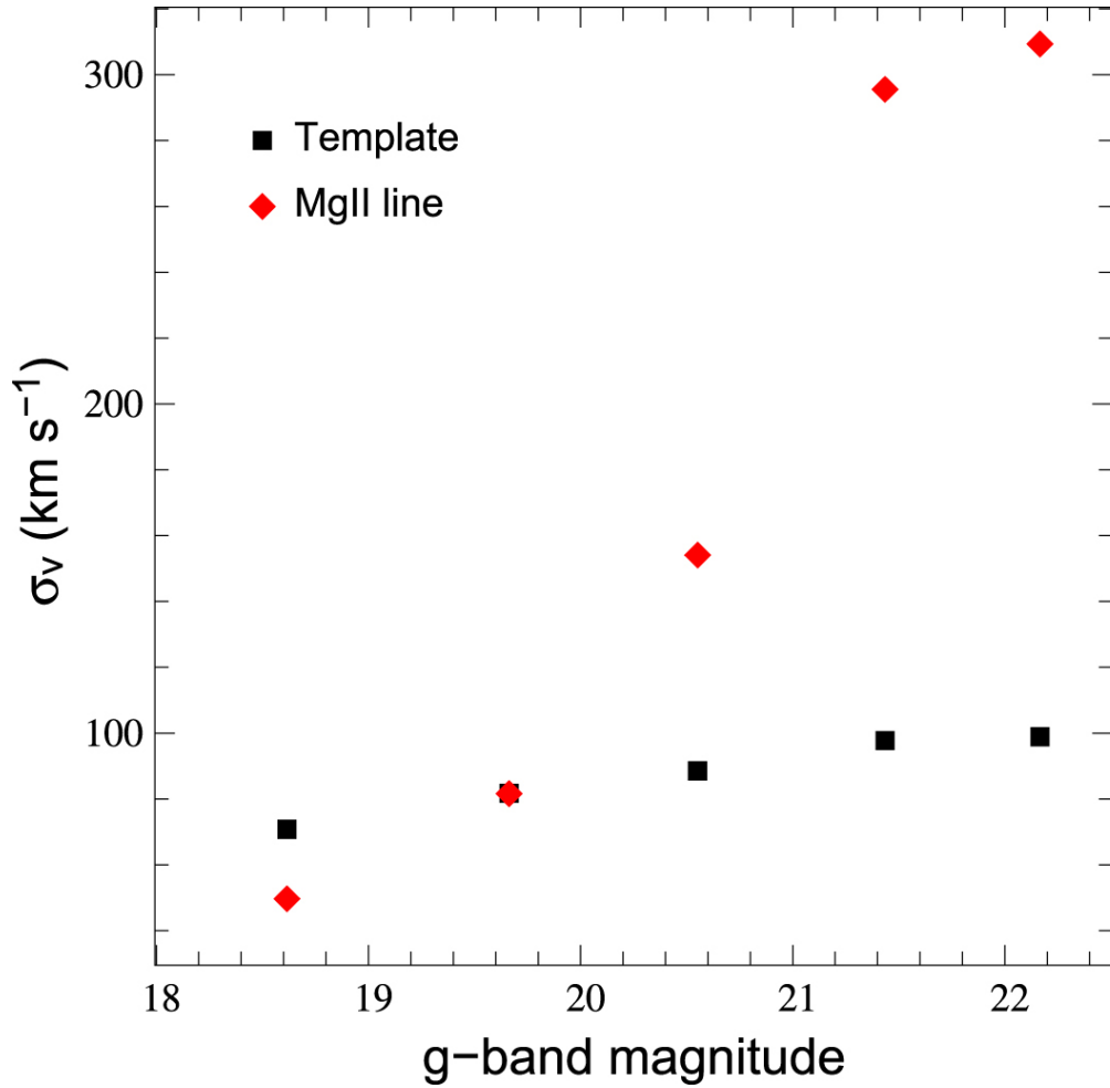
Figure 10. from THE SDSS-IV EXTENDED BARYON OSCILLATION SPECTROSCOPIC SURVEY: OVERVIEW AND EARLY DATA null 2016 AJ 151 44 doi:10.3847/0004-6256/151/2/44 https://dx.doi.org/10.3847/0004-6256/151/2/44 © 2016. The American Astronomical Society. All rights reserved.
