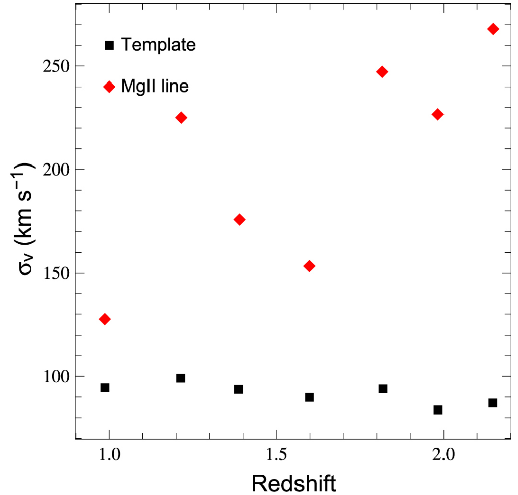
Figure 10. from THE SDSS-IV EXTENDED BARYON OSCILLATION SPECTROSCOPIC SURVEY: OVERVIEW AND EARLY DATA null 2016 AJ 151 44 doi:10.3847/0004-6256/151/2/44 https://dx.doi.org/10.3847/0004-6256/151/2/44 © 2016. The American Astronomical Society. All rights reserved.
