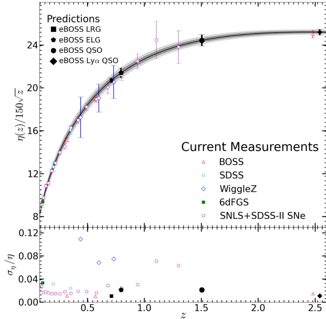
Figure 1. from THE SDSS-IV EXTENDED BARYON OSCILLATION SPECTROSCOPIC SURVEY: OVERVIEW AND EARLY DATA null 2016 AJ 151 44 doi:10.3847/0004-6256/151/2/44 https://dx.doi.org/10.3847/0004-6256/151/2/44 © 2016. The American Astronomical Society. All rights reserved.
