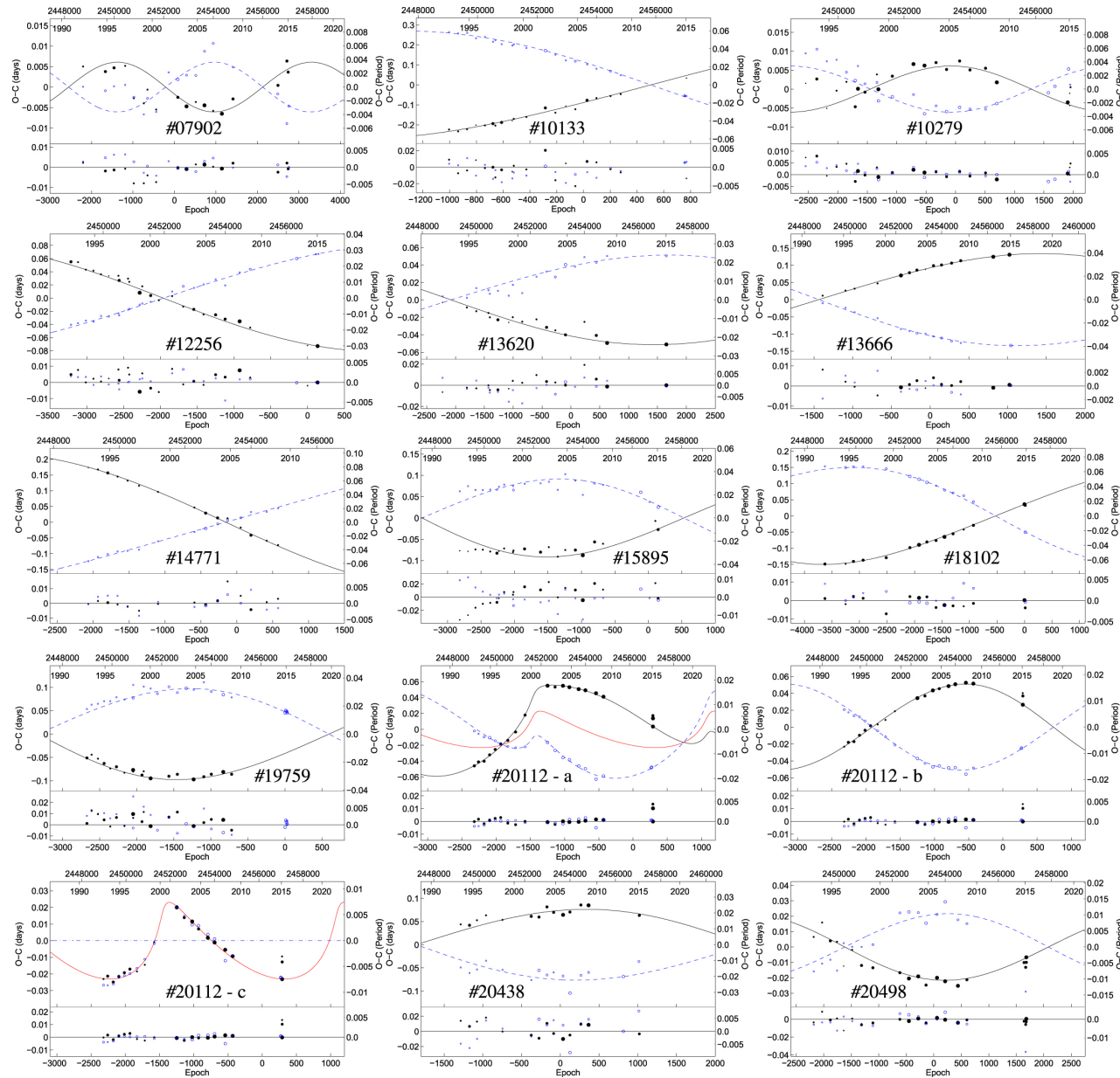
Figure 2. from APSIDAL MOTION AND A LIGHT CURVE SOLUTION FOR 13 LMC ECCENTRIC ECLIPSING BINARIES null 2015 AJ 150 183 doi:10.1088/0004-6256/150/6/183 https://dx.doi.org/10.1088/0004-6256/150/6/183
