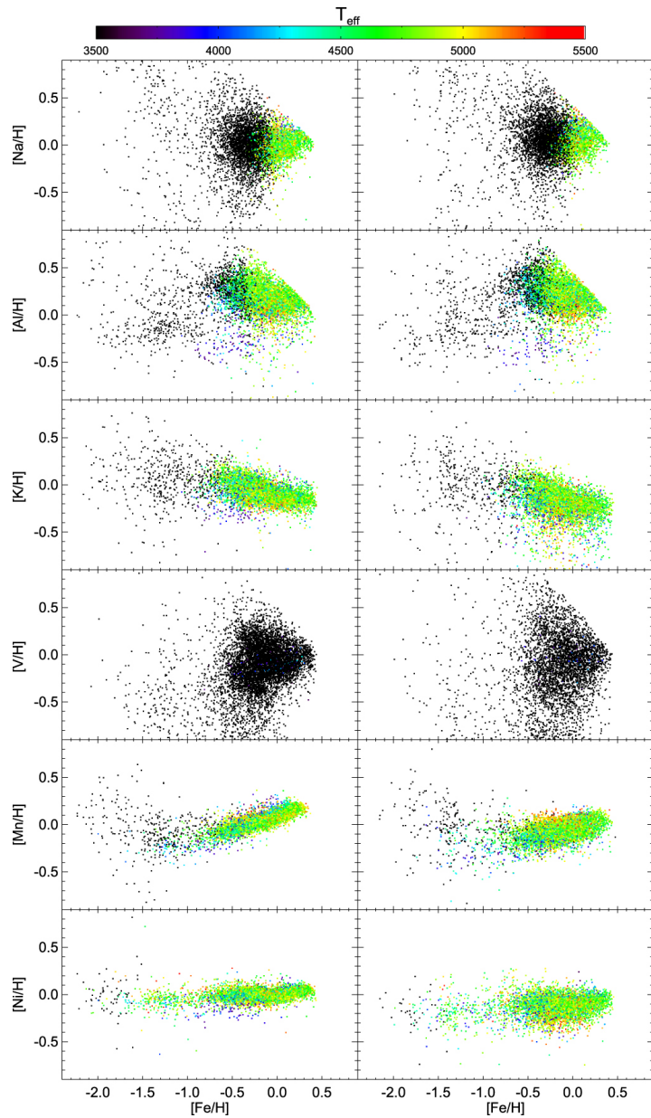
Figure 18. from ABUNDANCES, STELLAR PARAMETERS, AND SPECTRA FROM THE SDSS-III/APOGEE SURVEY null 2015 AJ 150 148 doi:10.1088/0004-6256/150/5/148 https://dx.doi.org/10.1088/0004-6256/150/5/148 © 2015. The American Astronomical Society. All rights reserved.
