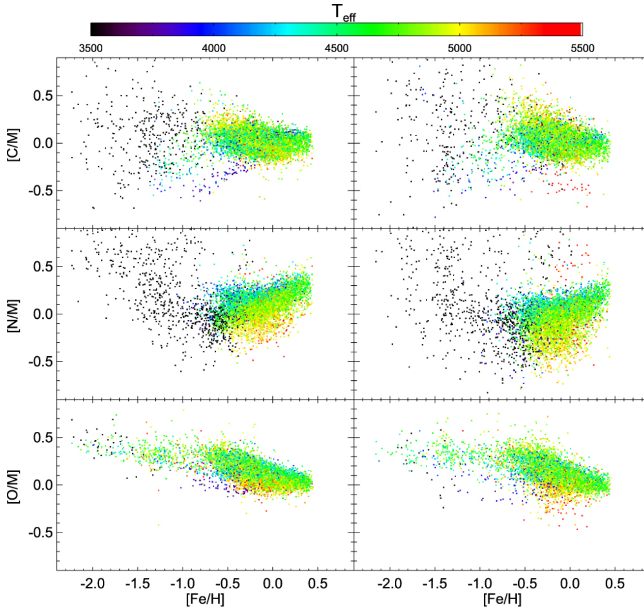
Figure 16. from ABUNDANCES, STELLAR PARAMETERS, AND SPECTRA FROM THE SDSS-III/APOGEE SURVEY null 2015 AJ 150 148 doi:10.1088/0004-6256/150/5/148 https://dx.doi.org/10.1088/0004-6256/150/5/148 © 2015. The American Astronomical Society. All rights reserved.
