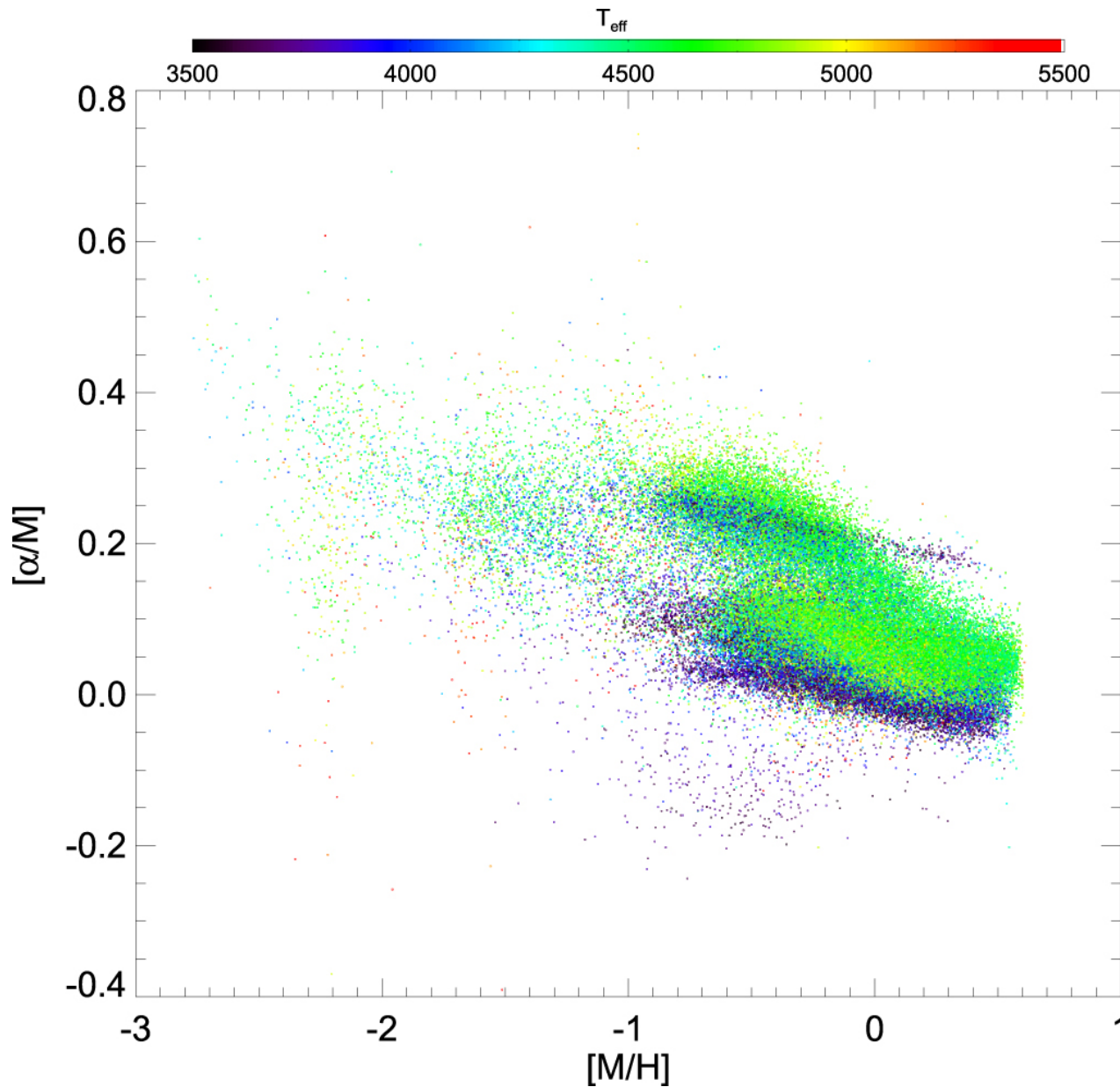
Figure 13. from ABUNDANCES, STELLAR PARAMETERS, AND SPECTRA FROM THE SDSS-III/APOGEE SURVEY null 2015 AJ 150 148 doi:10.1088/0004-6256/150/5/148 https://dx.doi.org/10.1088/0004-6256/150/5/148 © 2015. The American Astronomical Society. All rights reserved.
