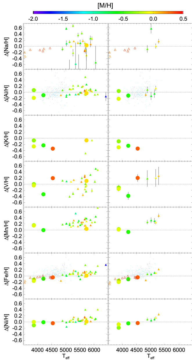
Figure 10. from ABUNDANCES, STELLAR PARAMETERS, AND SPECTRA FROM THE SDSS-III/APOGEE SURVEY null 2015 AJ 150 148 doi:10.1088/0004-6256/150/5/148 https://dx.doi.org/10.1088/0004-6256/150/5/148 © 2015. The American Astronomical Society. All rights reserved.
