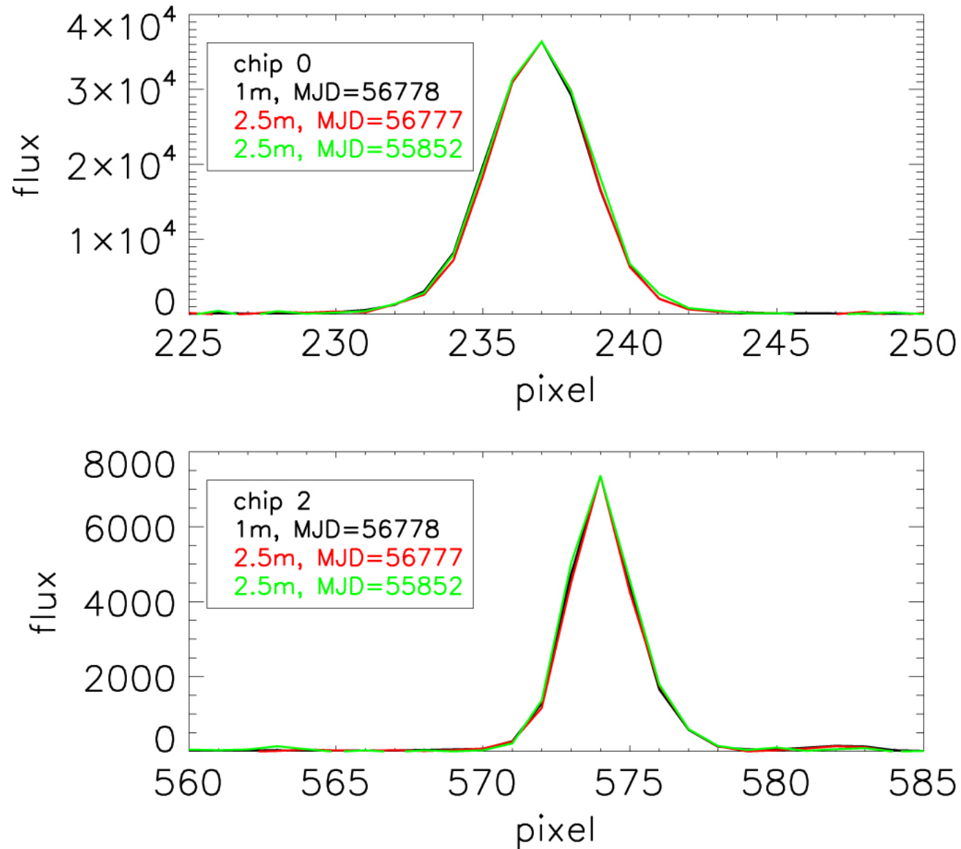
Figure 1. from ABUNDANCES, STELLAR PARAMETERS, AND SPECTRA FROM THE SDSS-III/APOGEE SURVEY null 2015 AJ 150 148 doi:10.1088/0004-6256/150/5/148 https://dx.doi.org/10.1088/0004-6256/150/5/148 © 2015. The American Astronomical Society. All rights reserved.
