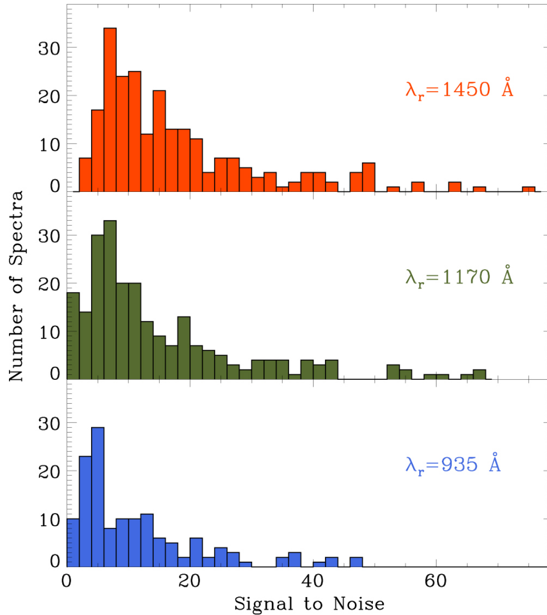
Figure 5. from THE FIRST DATA RELEASE OF THE KODIAQ SURVEY null 2015 AJ 150 111 doi:10.1088/0004-6256/150/4/111 https://dx.doi.org/10.1088/0004-6256/150/4/111 © 2015. The American Astronomical Society. All rights reserved.
