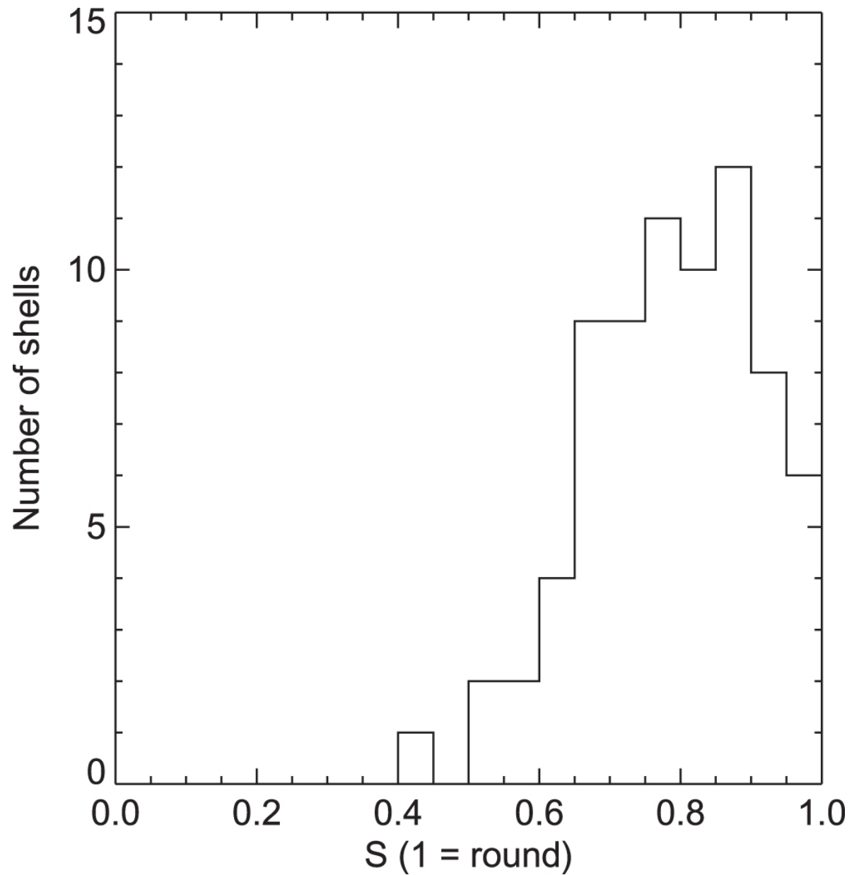
Figure 6. from INTERSTELLAR H I SHELLS IDENTIFIED IN THE SETHI SURVEY null 2015 AJ 149 189 doi:10.1088/0004-6256/149/6/189 https://dx.doi.org/10.1088/0004-6256/149/6/189 © 2015. The American Astronomical Society. All rights reserved.
