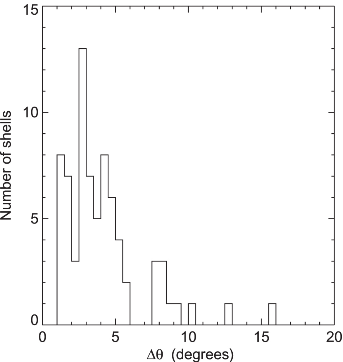
Figure 5. from INTERSTELLAR H I SHELLS IDENTIFIED IN THE SETHI SURVEY null 2015 AJ 149 189 doi:10.1088/0004-6256/149/6/189 https://dx.doi.org/10.1088/0004-6256/149/6/189 © 2015. The American Astronomical Society. All rights reserved.
