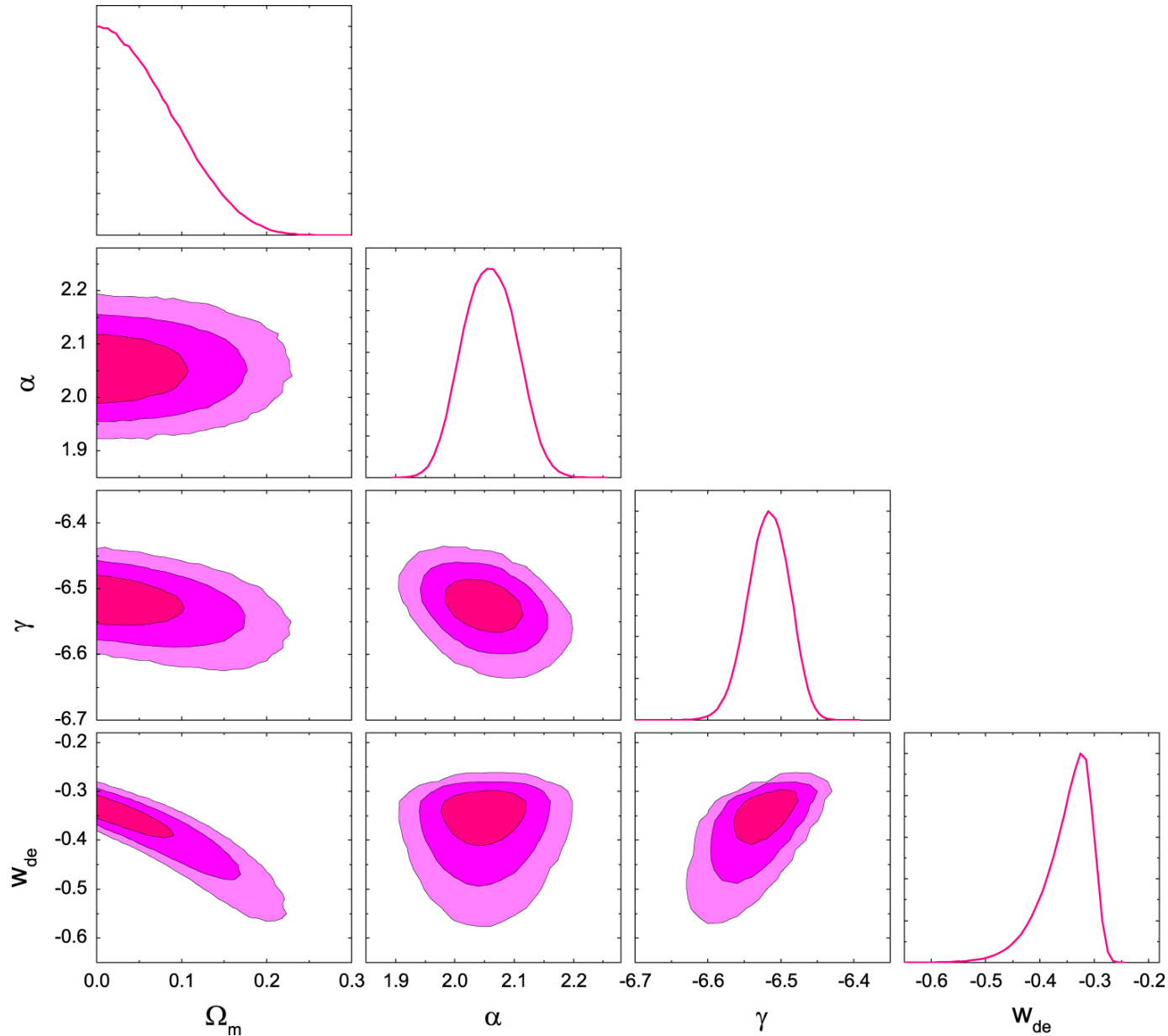
Figure 8. from TESTING COSMOLOGICAL MODELS WITH TYPE Ic SUPER LUMINOUS SUPERNOVAE null 2015 AJ 149 165 doi:10.1088/0004-6256/149/5/165 https://dx.doi.org/10.1088/0004-6256/149/5/165 © 2015. The American Astronomical Society. All rights reserved.
