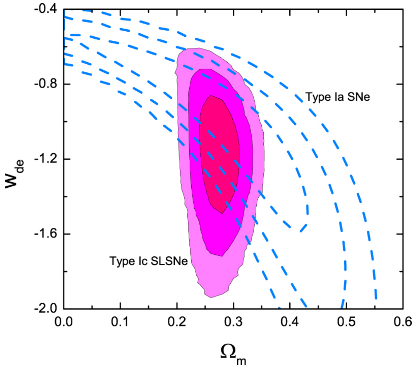
Figure 6. from TESTING COSMOLOGICAL MODELS WITH TYPE Ic SUPER LUMINOUS SUPERNOVAE null 2015 AJ 149 165 doi:10.1088/0004-6256/149/5/165 https://dx.doi.org/10.1088/0004-6256/149/5/165 © 2015. The American Astronomical Society. All rights reserved.
