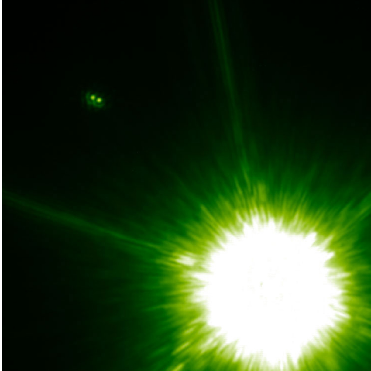
Figure 31. from BROWN DWARF BINARIES FROM DISINTEGRATING TRIPLE SYSTEMS null 2015 AJ 149 145 doi:10.1088/0004-6256/149/4/145 https://dx.doi.org/10.1088/0004-6256/149/4/145 © 2015. The American Astronomical Society. All rights reserved.
