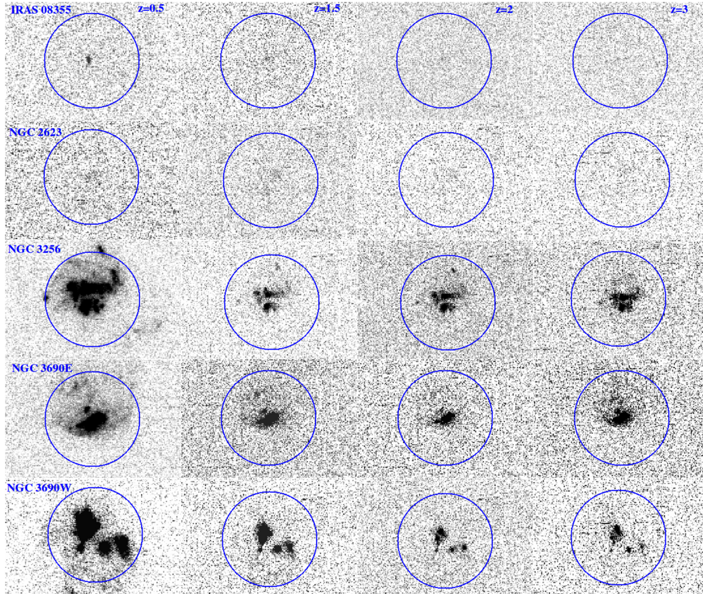
Figure 6. from THE FUV TO NEAR-IR MORPHOLOGIES OF LUMINOUS INFRARED GALAXIES IN THE GOALS SAMPLE null 2014 AJ 148 111 doi:10.1088/0004-6256/148/6/111 https://dx.doi.org/10.1088/0004-6256/148/6/111 © 2014. The American Astronomical Society. All rights reserved.
