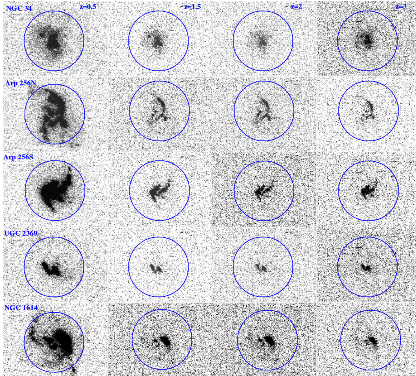
Figure 6. from THE FUV TO NEAR-IR MORPHOLOGIES OF LUMINOUS INFRARED GALAXIES IN THE GOALS SAMPLE null 2014 AJ 148 111 doi:10.1088/0004-6256/148/6/111 https://dx.doi.org/10.1088/0004-6256/148/6/111 © 2014. The American Astronomical Society. All rights reserved.
