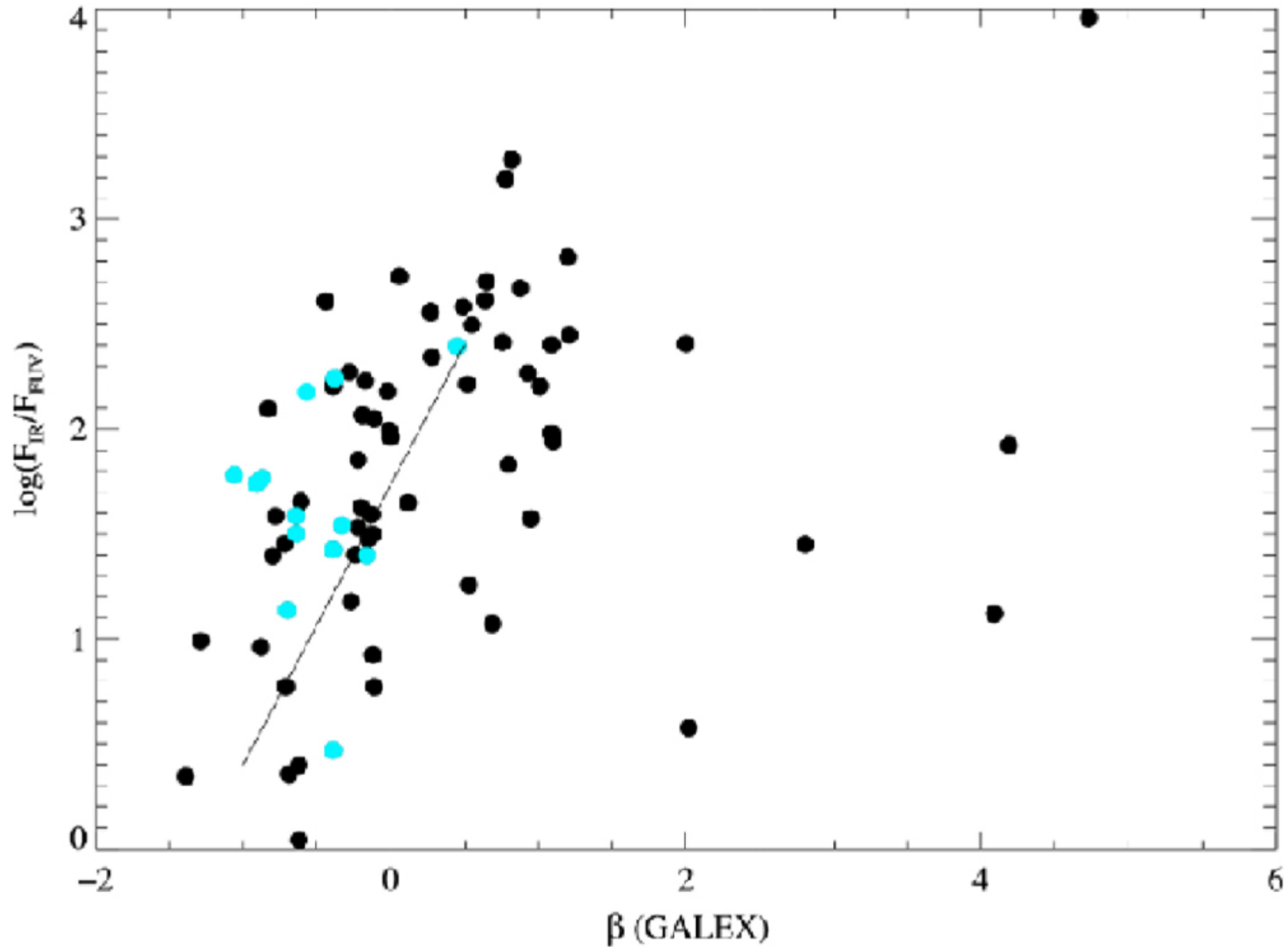
Figure 4. from THE FUV TO NEAR-IR MORPHOLOGIES OF LUMINOUS INFRARED GALAXIES IN THE GOALS SAMPLE null 2014 AJ 148 111 doi:10.1088/0004-6256/148/6/111 https://dx.doi.org/10.1088/0004-6256/148/6/111 © 2014. The American Astronomical Society. All rights reserved.
