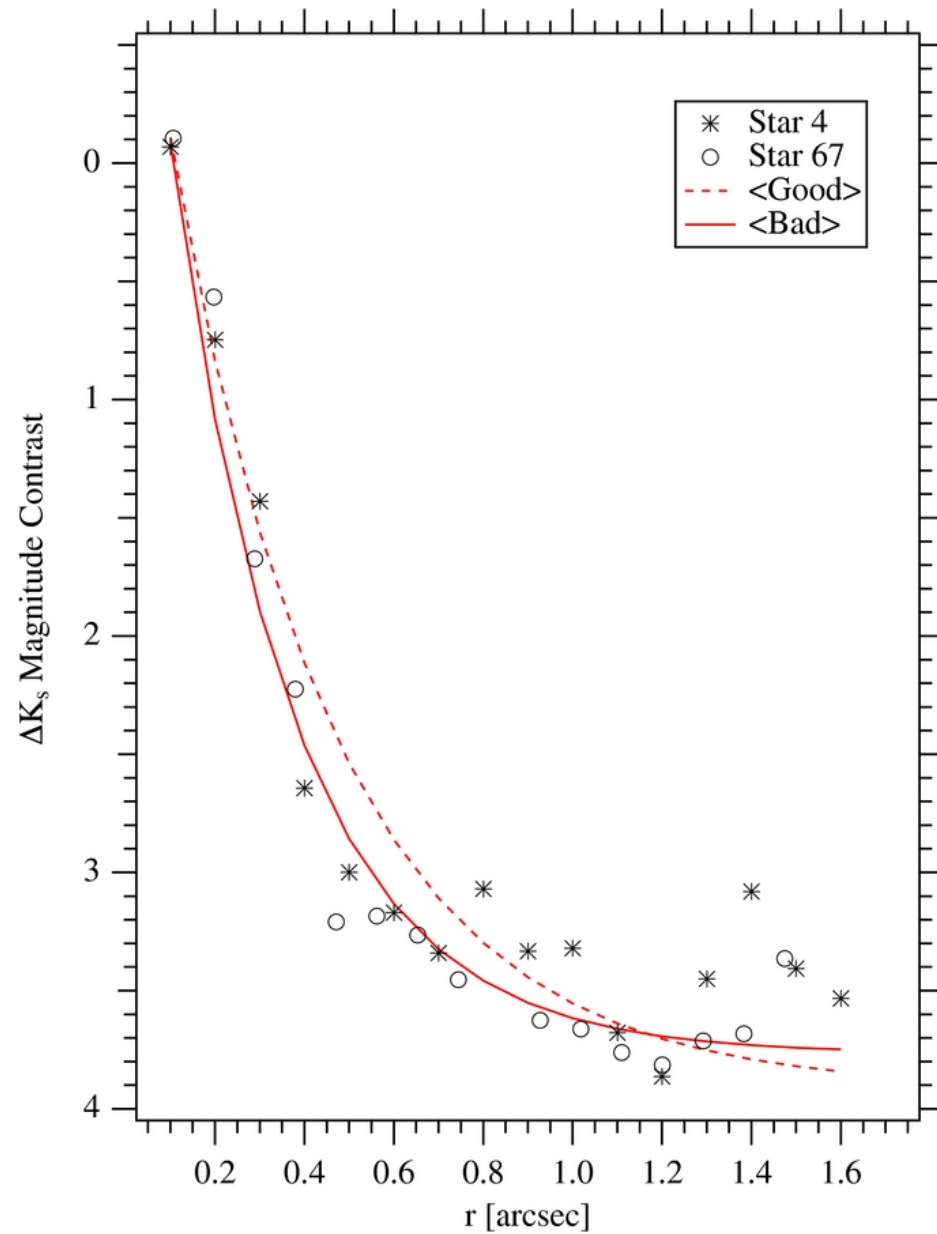
Figure 8. from A Technique to Derive Improved Proper Motions for Kepler Objects of Interest Benedict et al. 2014 AJ 148 108 doi:10.1088/0004-6256/148/6/108 https://dx.doi.org/10.1088/0004-6256/148/6/108 © 2014. The American Astronomical Society. All rights reserved.
