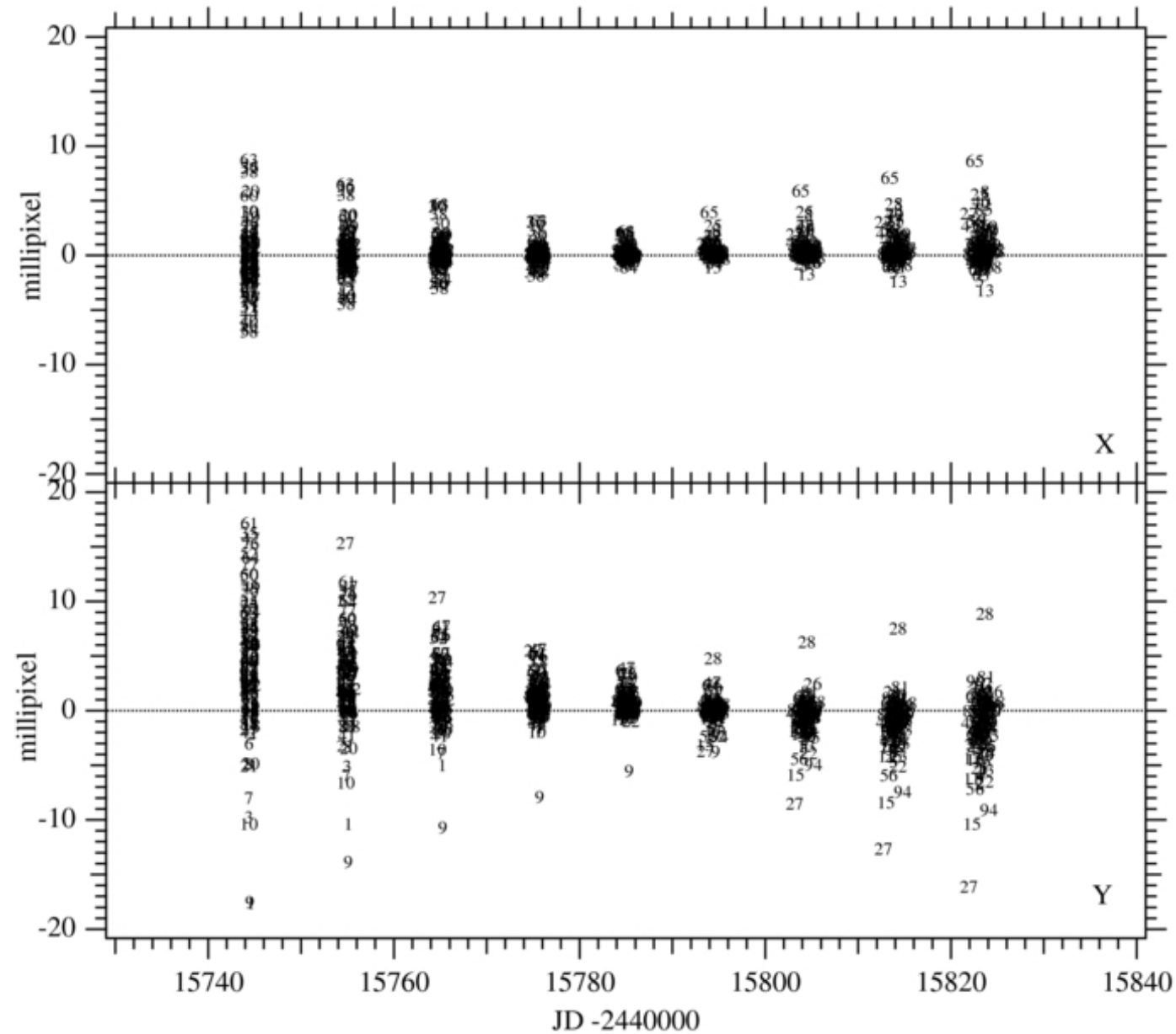
Figure 4. from A Technique to Derive Improved Proper Motions for Kepler Objects of Interest Benedict et al. 2014 AJ 148 108 doi:10.1088/0004-6256/148/6/108 https://dx.doi.org/10.1088/0004-6256/148/6/108 © 2014. The American Astronomical Society. All rights reserved.
