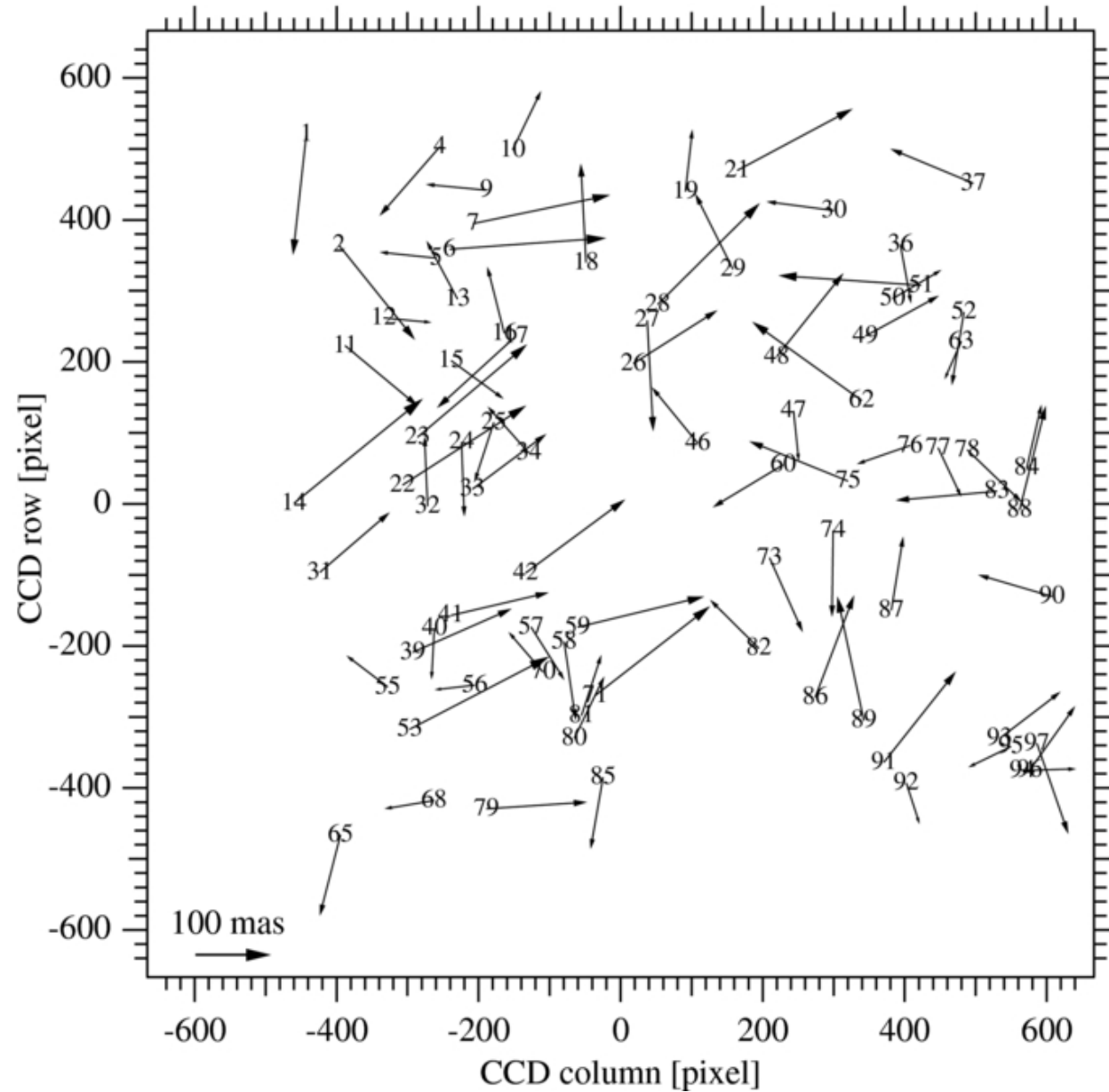
Figure 12. from A Technique to Derive Improved Proper Motions for Kepler Objects of Interest Benedict et al. 2014 AJ 148 108 doi:10.1088/0004-6256/148/6/108 https://dx.doi.org/10.1088/0004-6256/148/6/108 © 2014. The American Astronomical Society. All rights reserved.
