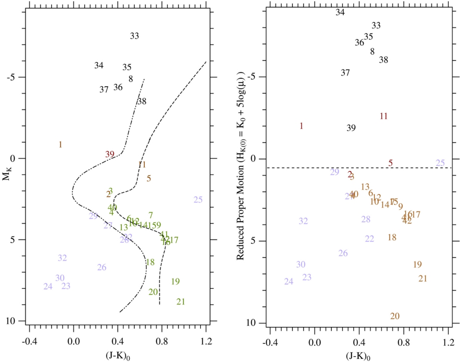
Figure 1. from A Technique to Derive Improved Proper Motions for Kepler Objects of Interest Benedict et al. 2014 AJ 148 108 doi:10.1088/0004-6256/148/6/108 https://dx.doi.org/10.1088/0004-6256/148/6/108 © 2014. The American Astronomical Society. All rights reserved.
