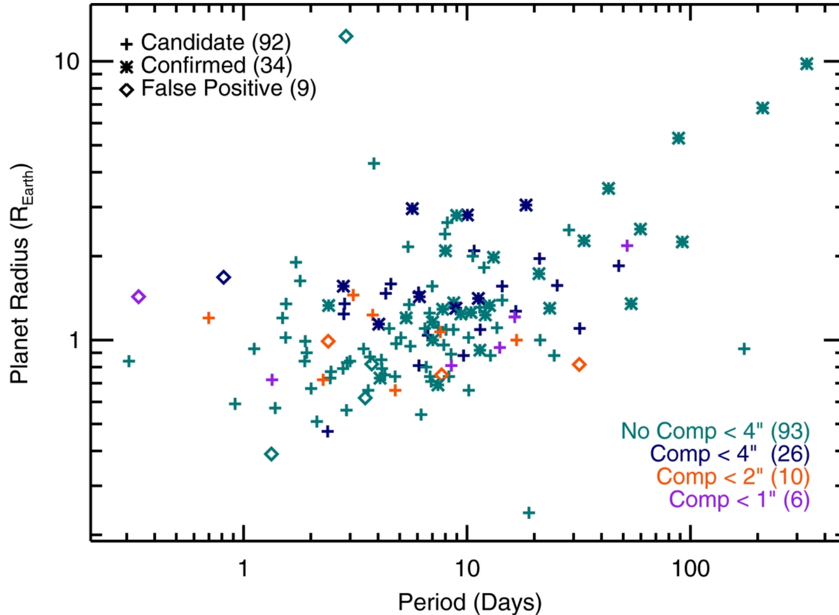
Figure 7. from Adaptive Optics Images. III. 87 Kepler Objects of Interest Dressing et al. 2014 AJ 148 78 doi:10.1088/0004-6256/148/5/78 https://dx.doi.org/10.1088/0004-6256/148/5/78 © 2014. The American Astronomical Society. All rights reserved.
