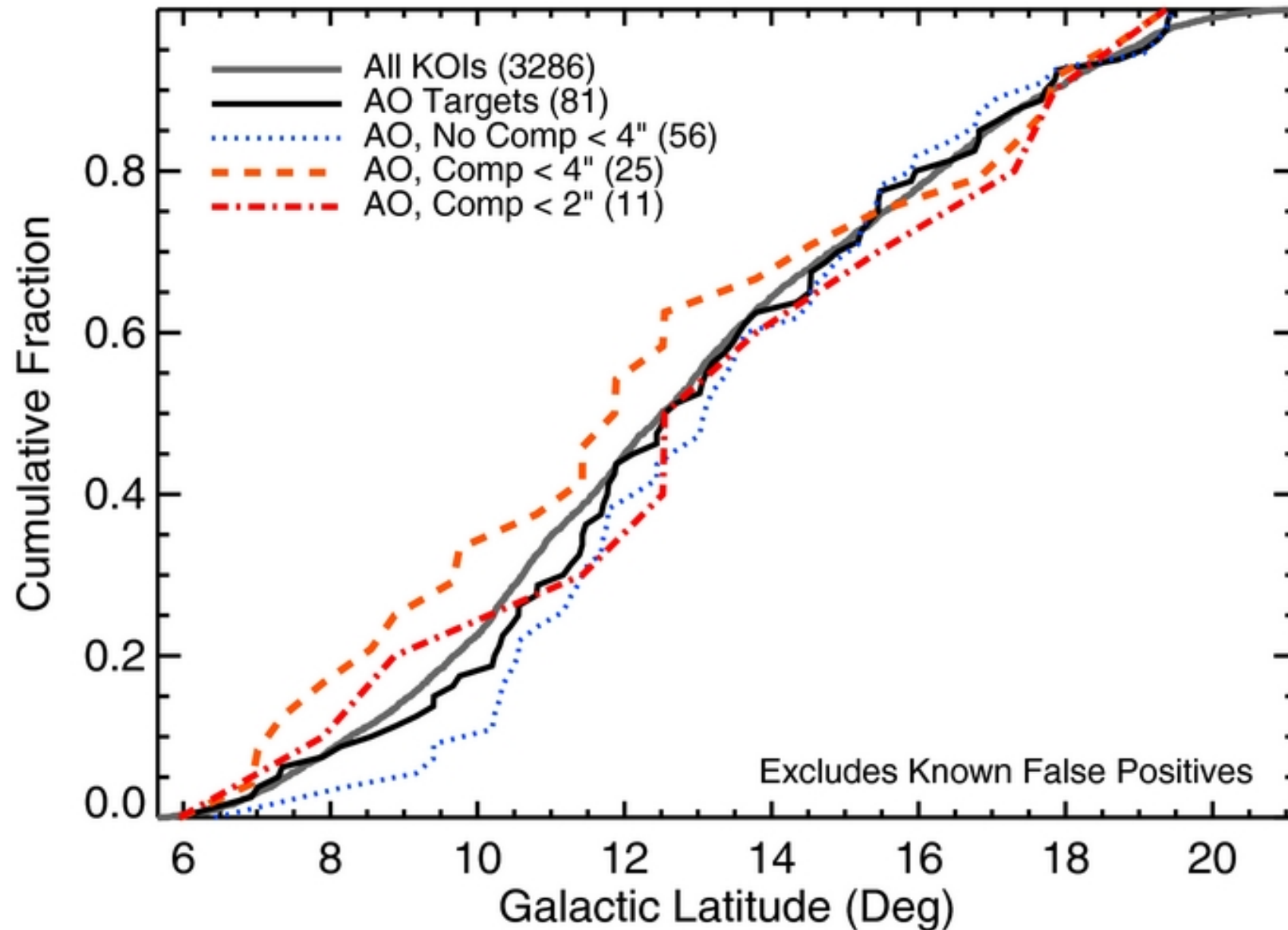
Figure 6. from Adaptive Optics Images. III. 87 Kepler Objects of Interest Dressing et al. 2014 AJ 148 78 doi:10.1088/0004-6256/148/5/78 https://dx.doi.org/10.1088/0004-6256/148/5/78 © 2014. The American Astronomical Society. All rights reserved.
