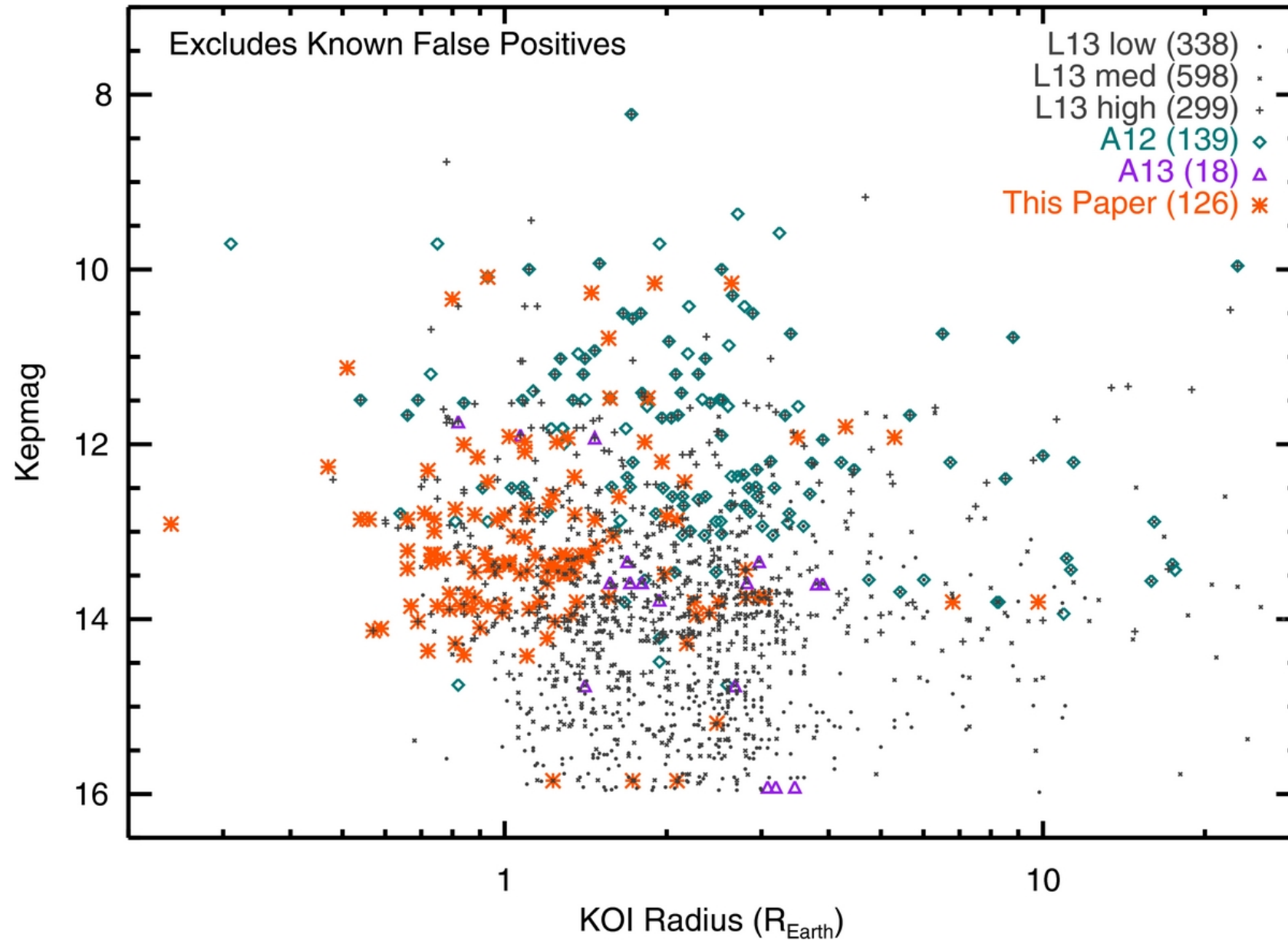
Figure 5. from Adaptive Optics Images. III. 87 Kepler Objects of Interest Dressing et al. 2014 AJ 148 78 doi:10.1088/0004-6256/148/5/78 https://dx.doi.org/10.1088/0004-6256/148/5/78 © 2014. The American Astronomical Society. All rights reserved.
