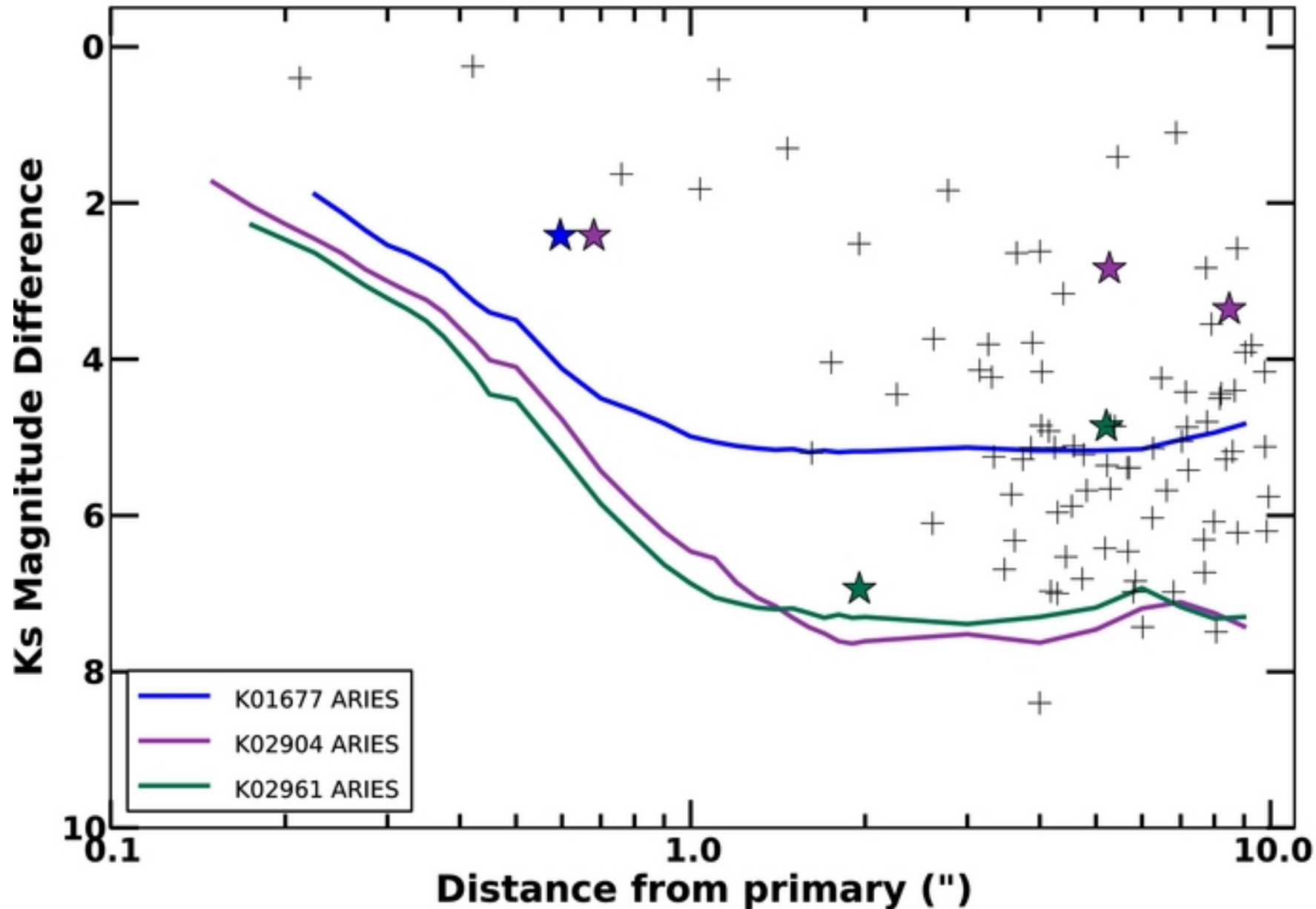
Figure 4. from Adaptive Optics Images. III. 87 Kepler Objects of Interest Dressing et al. 2014 AJ 148 78 doi:10.1088/0004-6256/148/5/78 https://dx.doi.org/10.1088/0004-6256/148/5/78 © 2014. The American Astronomical Society. All rights reserved.
