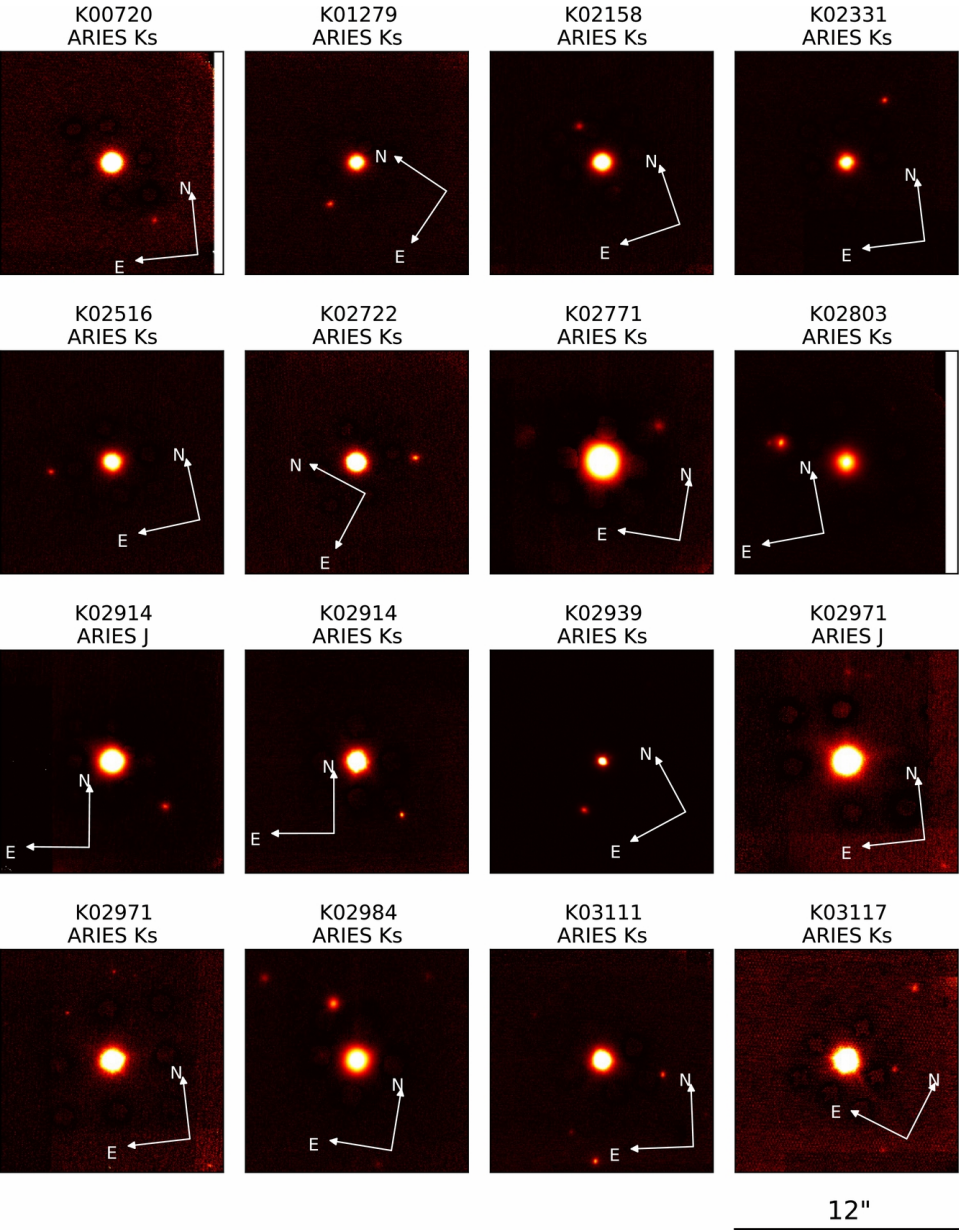
Figure 3. from Adaptive Optics Images. III. 87 Kepler Objects of Interest Dressing et al. 2014 AJ 148 78 doi:10.1088/0004-6256/148/5/78 https://dx.doi.org/10.1088/0004-6256/148/5/78 © 2014. The American Astronomical Society. All rights reserved.
