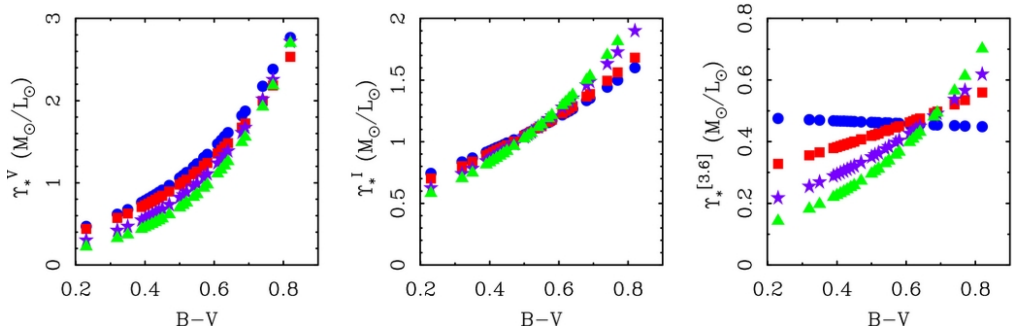
Figure 6. from Color-Mass-to-light-ratio Relations for Disk Galaxies McGaugh & Schombert 2014 AJ 148 77 doi:10.1088/0004-6256/148/5/77 https://dx.doi.org/10.1088/0004-6256/148/5/77 © 2014. The American Astronomical Society. All rights reserved.
