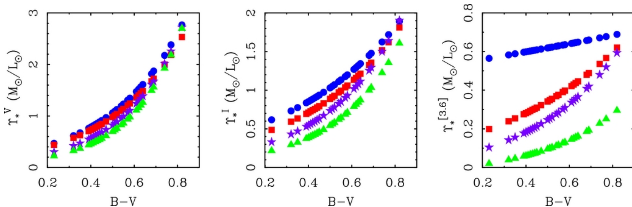
Figure 1. from Color-Mass-to-light-ratio Relations for Disk Galaxies McGaugh & Schombert 2014 AJ 148 77 doi:10.1088/0004-6256/148/5/77 https://dx.doi.org/10.1088/0004-6256/148/5/77 © 2014. The American Astronomical Society. All rights reserved.
