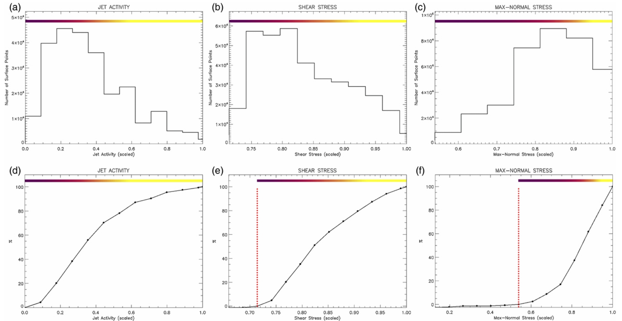
Figure 7. from How the Geysers, Tidal Stresses, and Thermal Emission across the South Polar Terrain of Enceladus are Related Porco, DiNino, & Nimmo 2014 AJ 148 45 doi:10.1088/0004-6256/148/3/45 https://dx.doi.org/10.1088/0004-6256/148/3/45 © 2014. The American Astronomical Society. All rights reserved.
